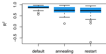
Figure 6: Distribution across 30 LON seeds of model R^2 on validation data (mean over 100 cross-validation iterations) with three ILS variants as the response variable. Predictors are the top three LON metrics obtained from feature selection
