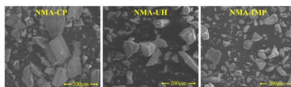
Fig. 1 – SEM images of calcined catalysts.
