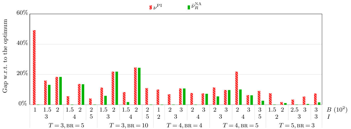
Figure 7 Quality of the bounds from the PI and LDDRs for small-size newsvendor instances
