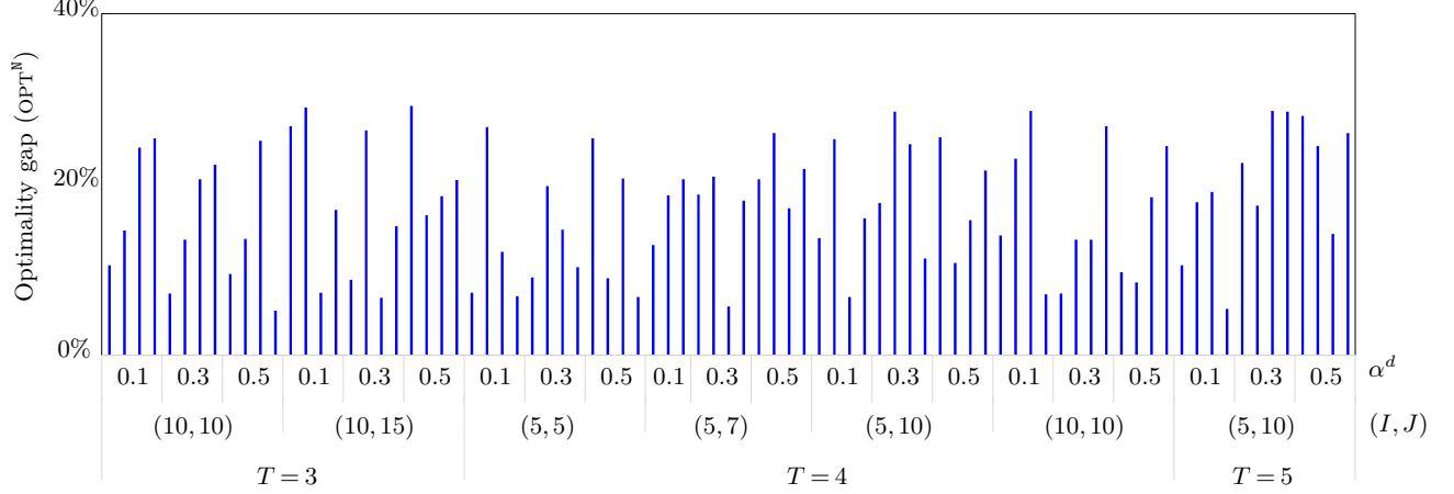
Figure 8 Optimality gaps for the location-transportation budgeted-uncertainty instances, between \nu^{2S-LDR} and \bar{\nu}_R^{NA} .
