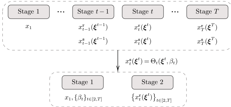
Figure 4 Two-stage decision rules
