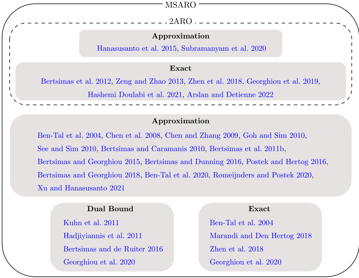
Figure 2 Solution methods for the MSARO
