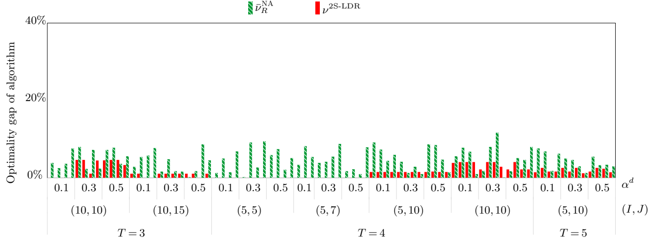
Figure 9 Optimality gaps of the solution algorithms for \nu^{2S-LDR} and \bar{\nu}_R^{NA} at convergence/interruption.
