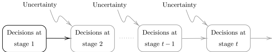
Figure 1 Sequential decision-making under uncertainty
