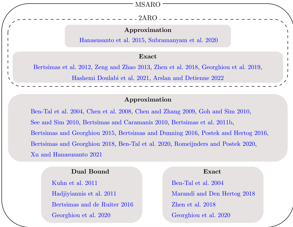
Figure 2 Solution methods for the MSARO
