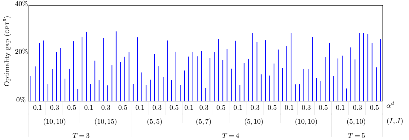
Figure 8 Optimality gaps for the location-transportation budgeted-uncertainty instances, between \nu^{2S-LDR} and \bar{\nu}_R^{NA} .
