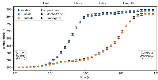
Fig. 7. Validation of the propagator implementation (triangles) against a Monte Carlo simulation (circles) on the computation of the lower-room probe temperature and its uncertainty (as in Fig. 6), which are similar in both cases.
