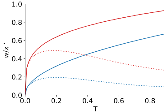
Figure 8: Lateral extent of the thickness heterogeneity normalized by the characteristic length scale x^* of the corresponding regime as a function of the normalized time T in the capillarity (red lines) and gravity-driven (blue lines) limits. The curves correspond to different reference states for linearization: under the mask \alpha = 0 (full lines) and away from the mask \alpha = \nu + 3 (dotted lines)
