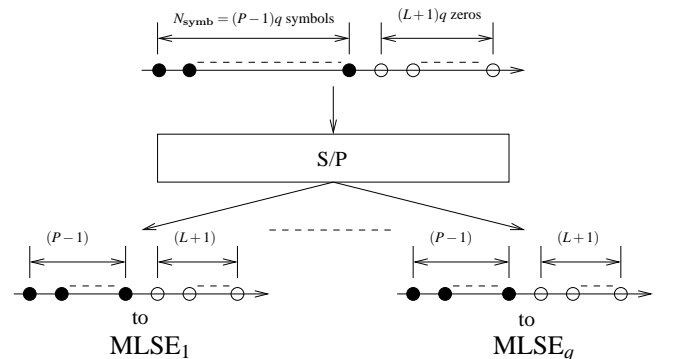
Figure 5: The ZP signal frame structure before and after serial to parallel conversion
