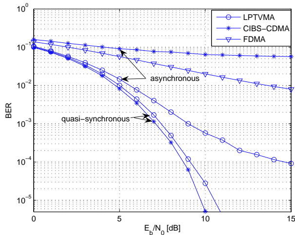
Figure 7: The performances of the LPTVMA system compared to CIBS-CDMA and FDMA systems
