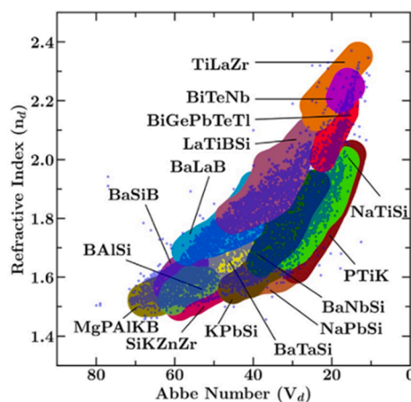
Fig. 24. An Abbe diagram for the visible wavelengths generated using the machine learning models. Points represent the experimental data, and the colored regions indicate the range of properties achievable using respective glass compositions (Reproduced from Ref. [287] with permission from American Ceramic Society).
