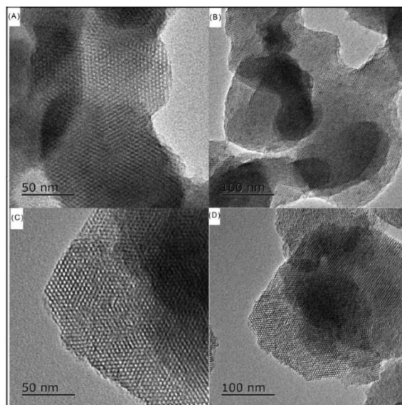
Fig. 31. TEM micrographs of different samples prepared by changing xSi/Ti-MCM-41TTe1 (A) & (B) for x=10, (C) & (D) for x=60 (Liu et al. 2017).
