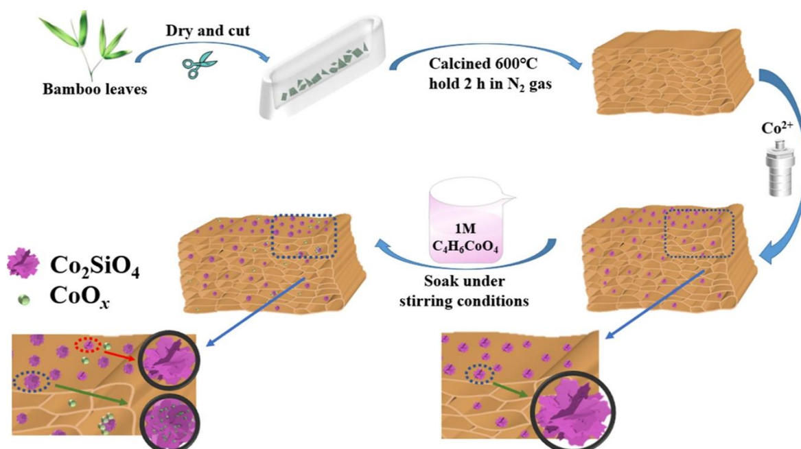
Fig. 29. Synthetic route and SEM images of C/CoSi and Co-rich C/CoSi: (a) Synthetic route of C/CoSi and Co-rich C/CoSi (Pei et al. 2022).
