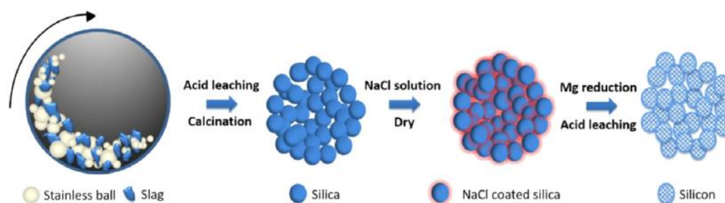
Fig. 46. Scheme of the method to prepare porous silicon from sodium slag (Huang et al. 2018).
