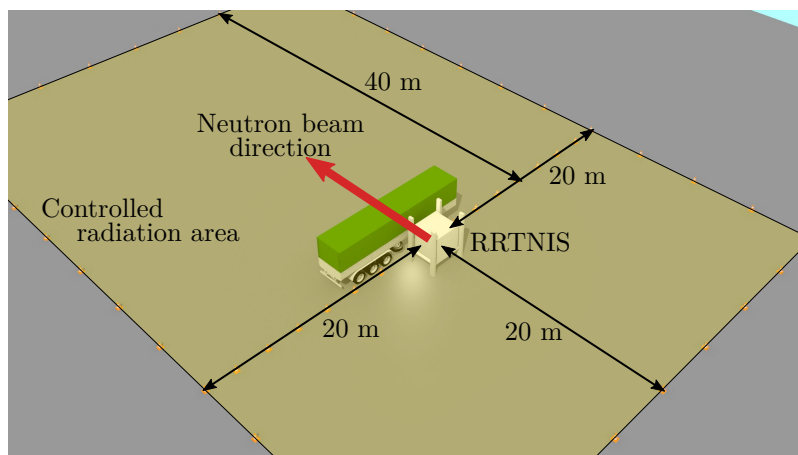
Slika 5: Diagram of the RRTNIS installation and controlled radiation area (40 m x 60 m) at the Rotterdam seaport test facility of DCA.
