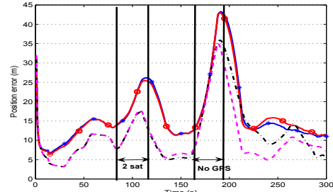
Figure 6: Position errors for urban scenario. (a) GPS/WSS approach with EKF and UKF (solid lines with \circ and \ast ). (b) GPS/INS/WSS approach with EKF (dash-dotted) and UKF (dotted lines).
