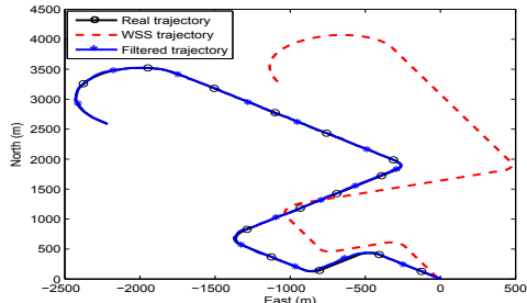
Figure 2: Example of an actual and estimated trajectory (GPS/WSS).
