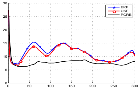
Figure 3: Horizontal position errors (GPS/WSS).
