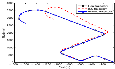
Figure 4: Actual and estimated trajectories (GPS/INS/WSS).
