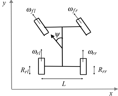
Figure 1: Illustration of WSS definition.
