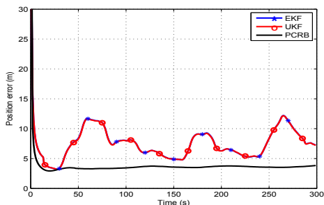
Figure 5: Horizontal position errors (GPS/INS/WSS).
