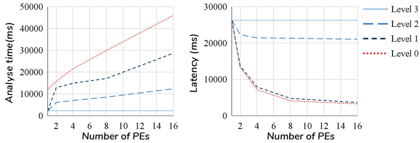
Fig. 7. Comparison of analysis time and latency between the classical flattening approach and three configurations of SCAPE method on Stereo application on several architectures
