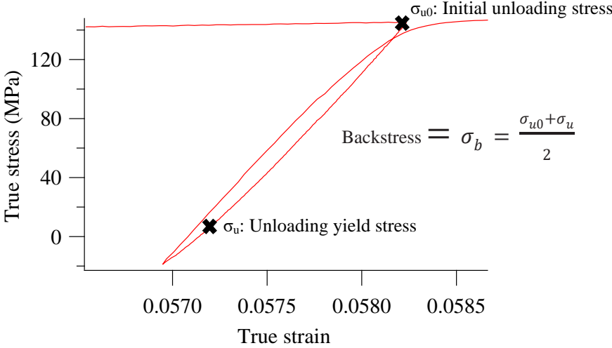
Fig. 2. (a) Pure Cu loading-unloading curve, (b) test specimen and (c) backstress calculation [18], [19]
