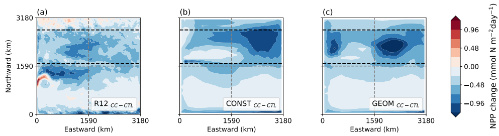
Figure 11: Raw differences of the vertically integrated Net Primary Production (NPP, \text{mmol N m}^{-2} \text{day}^{-1} , where N is the nitrogen currency) between the climate change scenario and the control scenario (Fig. 5a, b, c) for (a) R12, (b) CONST and (c) GEOM. The area enclosed by black dashed lines denote the boundaries of the subpolar gyre box mentioned in text.
