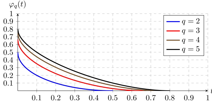
FIGURE 1. The function \varphi_q(t) for several values of q . Note that the case q=2 corresponds to the function \varphi(t) of (5).
