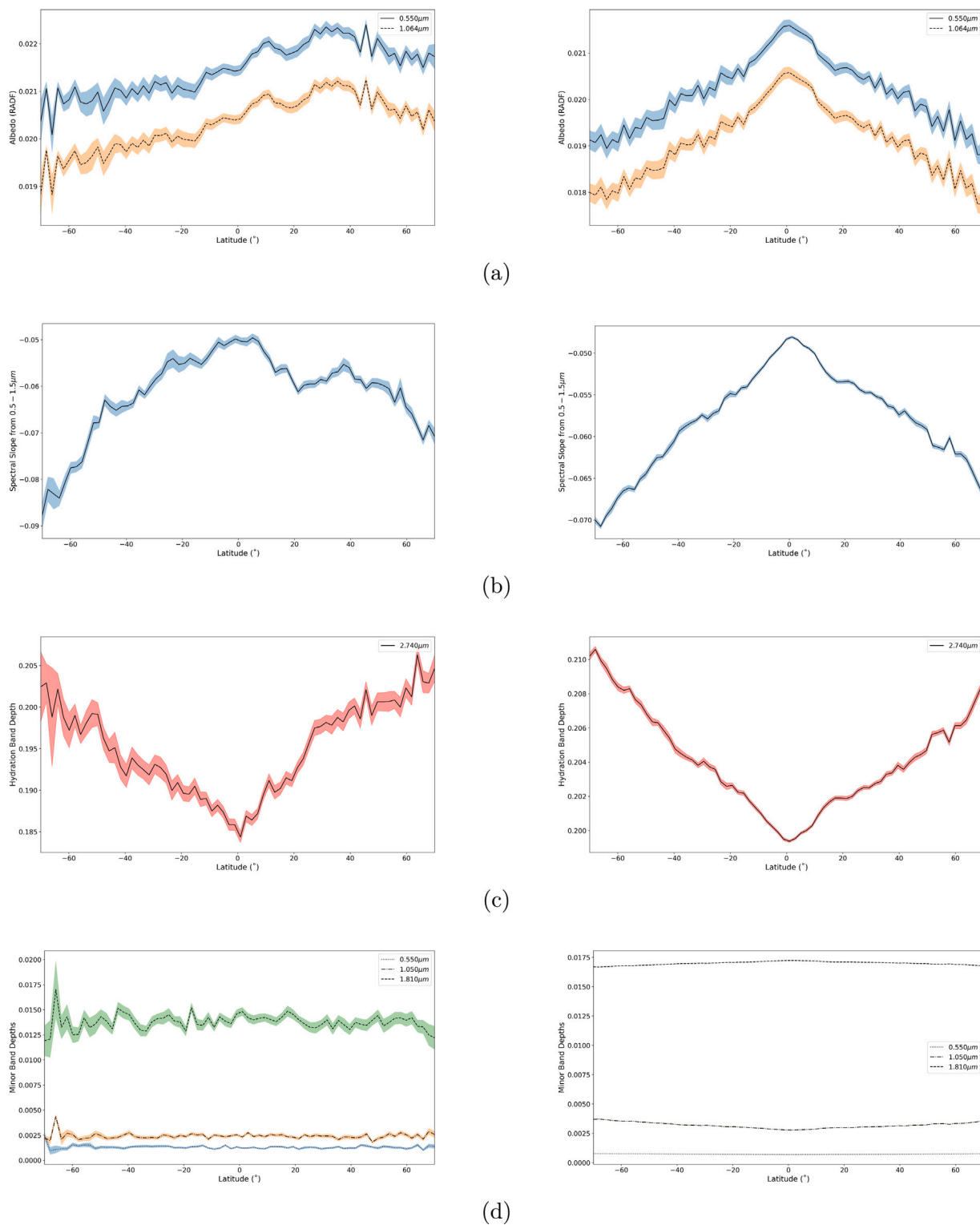
Fig. 6. Benu (a) albedo, (b) spectral slope, (c) 2.74 \mu\text{m} hydration band depth, and (d) minor band depth averages are calculated for 2^\circ latitudinal bins using regionally photometrically corrected OVIRS data from Li et al. (2021) (left) and photometric model radiance factor calculated using the McEwen model from Zou et al. (2021) (right). In each panel, the shaded area represents standard error of the mean. (For interpretation of the references to color in this figure legend, the reader is referred to the web version of this article.)
