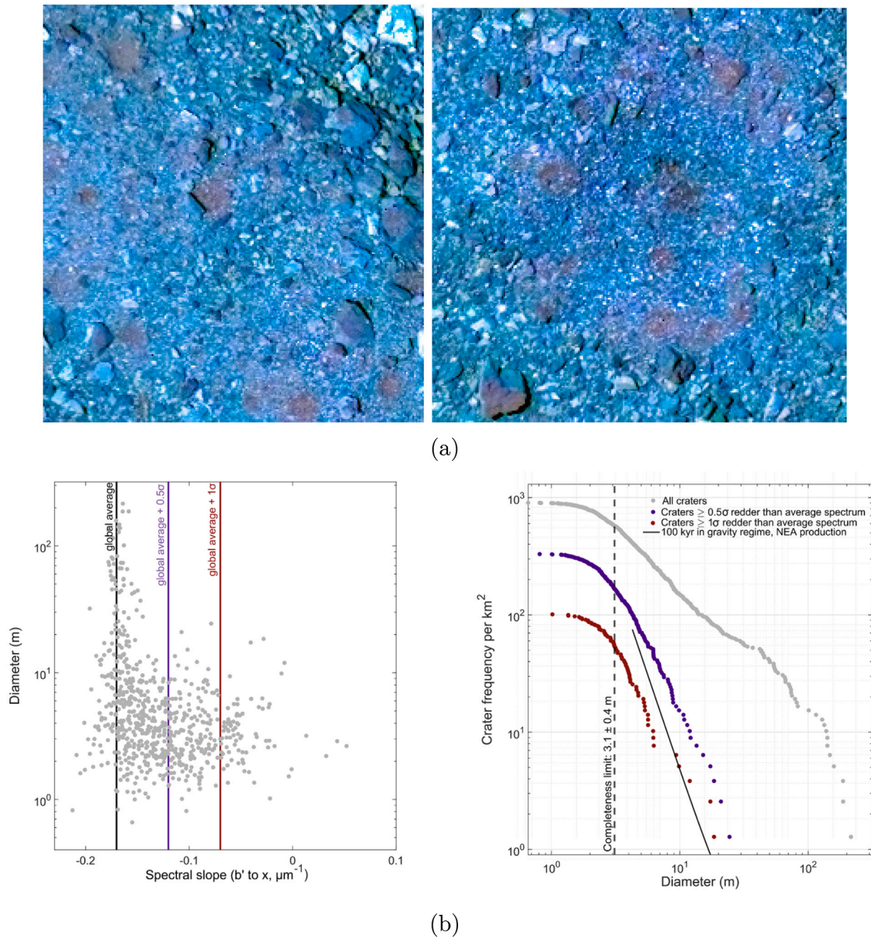
Fig. 1. (a) shows examples of the small red-colored craters found on Bennu, and (b) shows statistical distributions of crater diameters. The red circular depressions are all craters less than 10m in diameter (top left). The right frame encloses an older crater that is superimposed by the younger red craters. This shows that over time, crater colors eventually blend into the average blue-ish color of Bennu’s global materials. (For interpretation of the references to color in this figure legend, the reader is referred to the web version of this article.)
