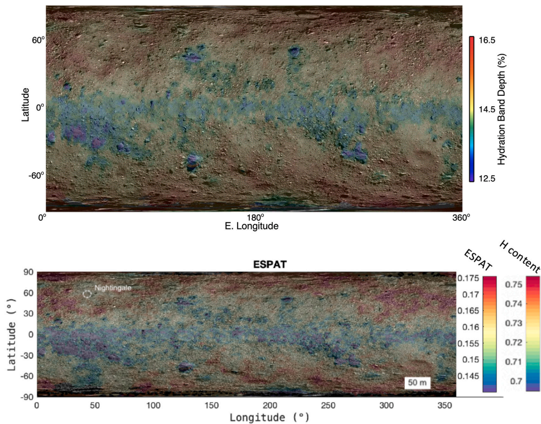
Fig. 3. The top panel shows a 2.7 \mu\text{m} band depth map from OVIRS measurements, reproduced from Simon et al. (2020a) . The bottom panel shows an ESPAT map of Bennu at 2.7 \mu\text{m} adapted from Praet et al. (2021) : spectral data at 20 m/footprint are converted to ESPAT and corresponding H content. This projection shows longitudes from 0° to 360° longitude. Both maps are overlain on the global image-mosaic basemap of Bennu ( Bennett et al., 2021 ). (For interpretation of the references to color in this figure legend, the reader is referred to the web version of this article.)
