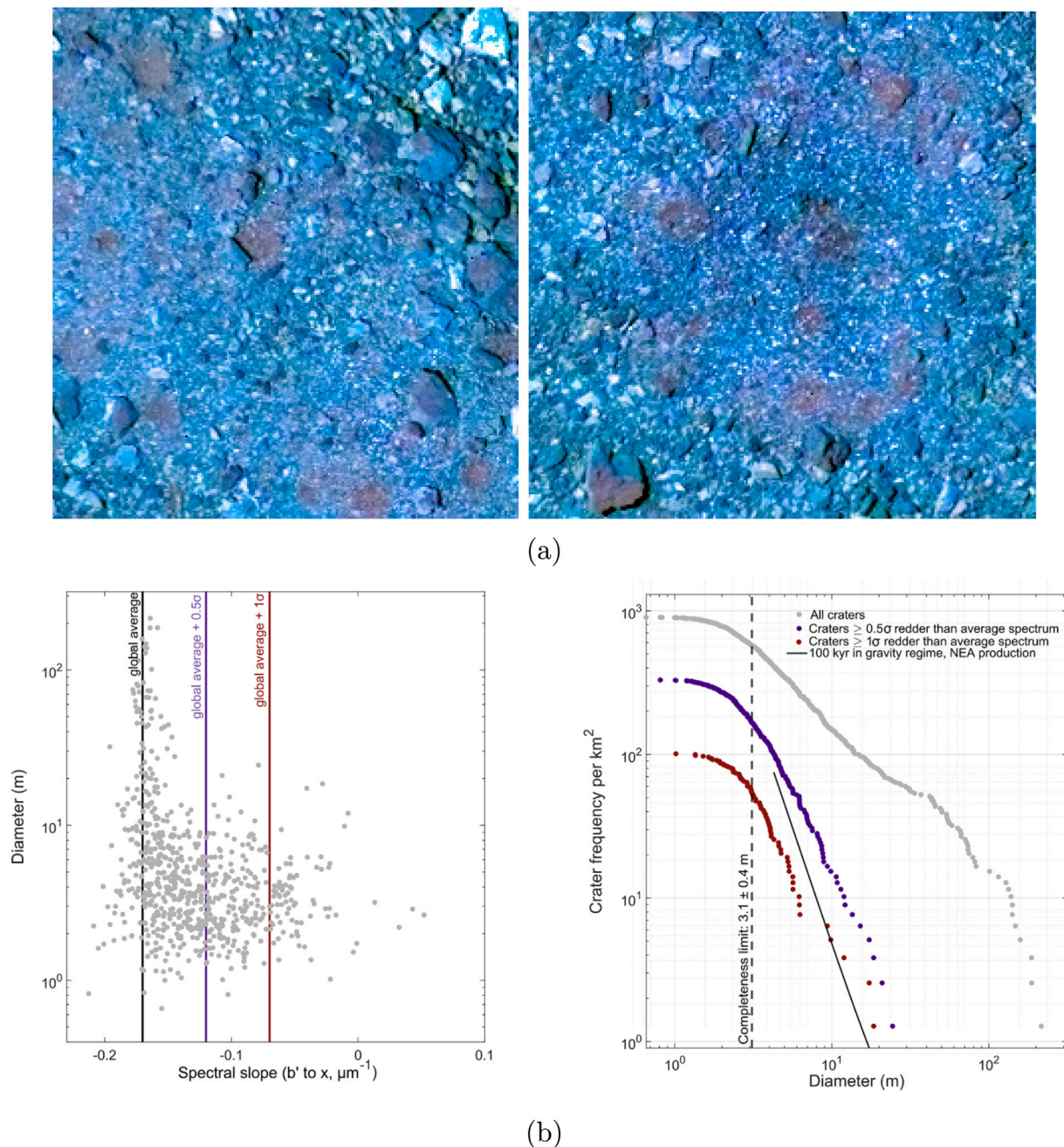
Fig. 1. (a) shows examples of the small red-colored craters found on Bennu, and (b) shows statistical distributions of crater diameters. The red circular depressions are all craters less than 10m in diameter (top left). The right frame encloses an older crater that is superimposed by the younger red craters. This shows that over time, crater colors eventually blend into the average blue-ish color of Bennu’s global materials. (For interpretation of the references to color in this figure legend, the reader is referred to the web version of this article.)
