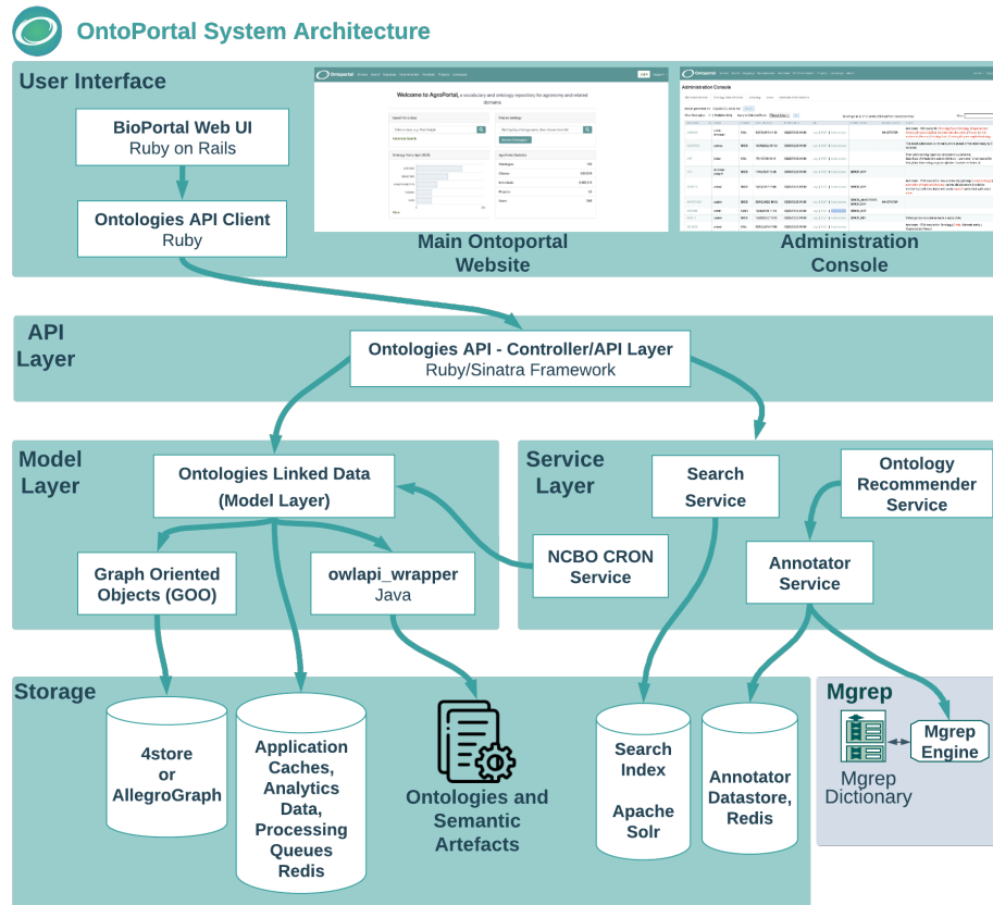
Fig. 2. OntoPortal system architecture.
