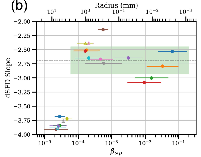
corresponding particle radius (assuming a density of 3500 kg/m 3 ) on the top axis. Filled circles are derived from the main tail, open triangles from the secondary tail. The horizontal error bars represent the range of \beta_{srp} covered by the corresponding tail profile. The colors of symbols correspond to the colors of profiles in panel (a). The slope values from the outer section have \beta_{srp} higher than 1 \times 10^{-4} , and those from the inner section correspond to \beta_{srp} between 1 \times 10^{-4} and 1 \times 10^{-5} . The dashed horizontal line is the average -2.7 for the outer sections, and the green shaded area represents the standard deviation.
