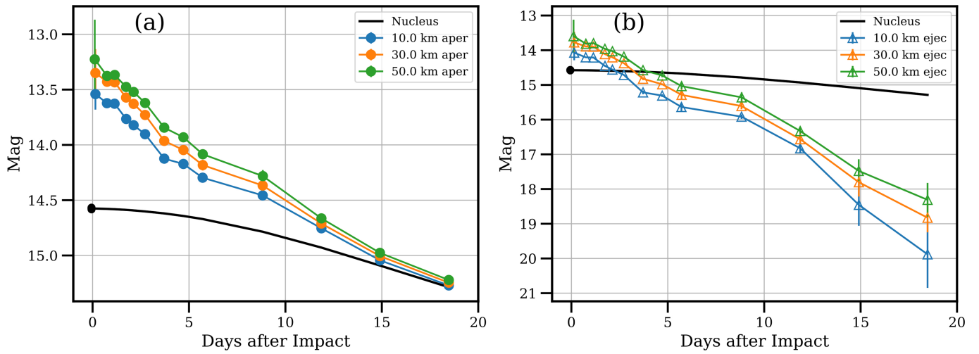
Extended Data Fig. 4 | Brightness evolutions of Didymos and the ejecta.
