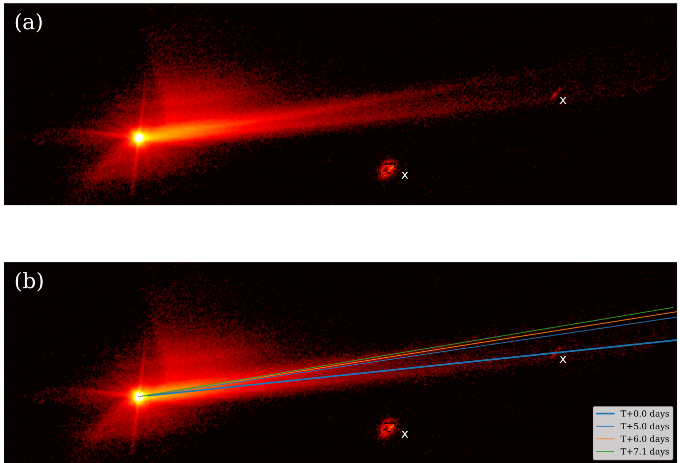
Extended Data Fig. 6 | Synchrone analysis of the main tail and the secondary tail. (a) Image taken at T+11.86 days is displayed in logarithmic brightness stretch. North is up and east to the left. The features marked by "x" are artifacts from a background object and a cosmic ray hit. (b) Same image as in (a) but with
