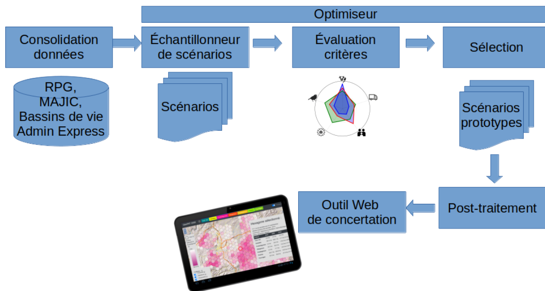
Figure 3: Architecture logicielle
