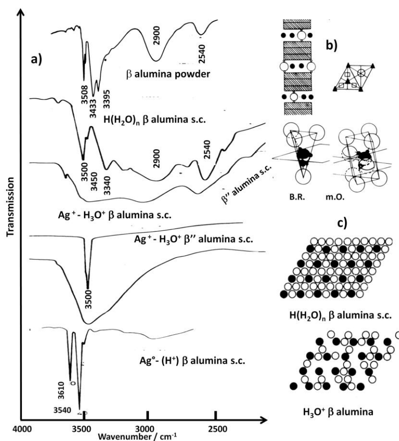
Fig. 1. Representative IR signatures of O-H, H 3 O + and H 5 O 2 + /H 7 O 3 + species in β alumina (a), schematic of the structure (b, with view of the Beever-Ross and middle-oxygen sites; black circle: oxonium ion; open circle: oxygen ion) and sketch of the site occupation in the conducting plane. In a), from the top spectra recorded using a dispersion of powdered partially hydrated oxonium β alumina single crystal in fluorolube ® mull in-between two CaF 2 wafers, comparison between the spectra of single crystal of β and β'' alumina phase, comparison of the spectra of single crystal of oxonium β and β'' alumina after partial ion exchange of ~30% of oxonium ions with silver ions [19]. Reliable relationship established between vibrational parameters (center of gravity of stretching band, bandwidth) and crystallographic data (O-H...X donor-acceptor distance)[16] allows determination of the H-bond distance with neighboring proton acceptors.[10,19]
