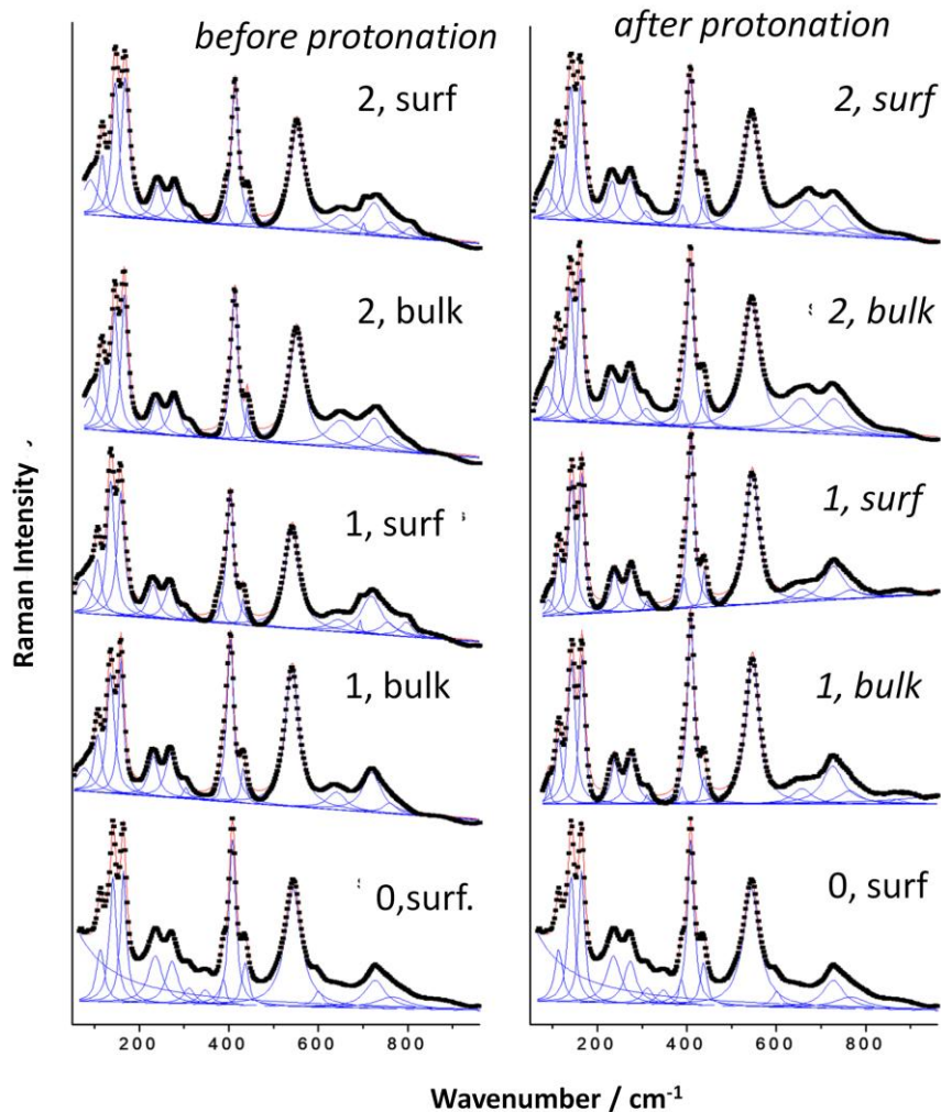
Fig. 3. Comparison of Raman spectra recorded on a dense sintered \text{SrZr}_{0.9}\text{Er}_{0.1}\text{O}_{3-\delta} ceramic (>98% of the theoretical density), at the surface (surf) and in the core after breakage (bulk) before protonation with those recorded after protonation in an autoclave at 500°C under 40 bar \text{H}_2\text{O} for a few days. The composition of protonated ceramic is \text{H}_{0.02}\text{SrZr}_{0.9}\text{Er}_{0.1}\text{O}_{3-\delta}
