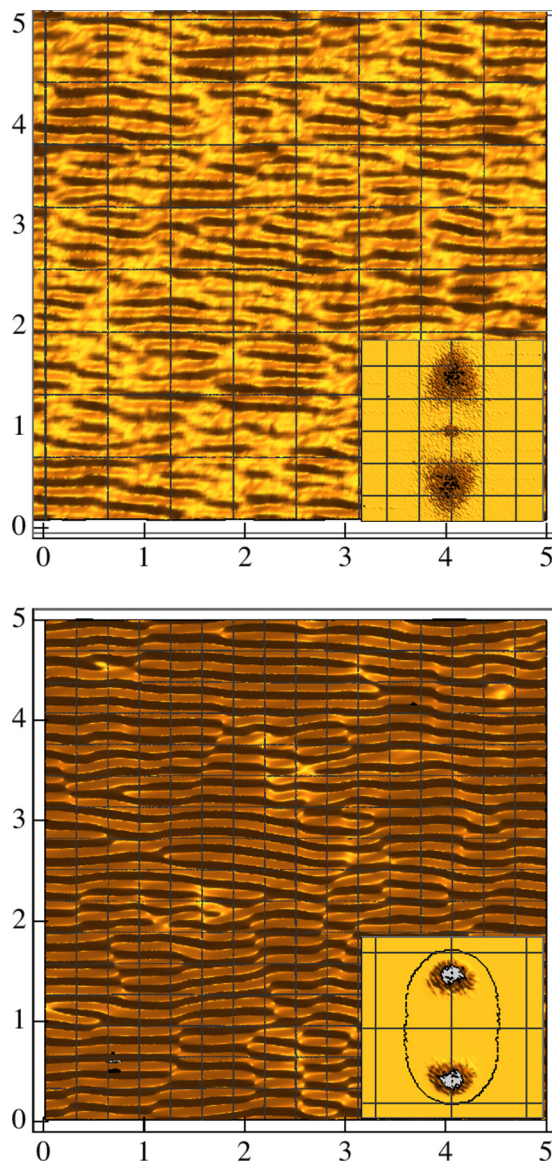
FIG. 7. (Left) Large-scale AFM image of the growth on a 10^\circ off substrate for a composition x=0.23 . (Right) Integration of the evolution equation (9) with an in-plane asymmetry \eta=0.36 . In both images, distances are given in micrometers.
