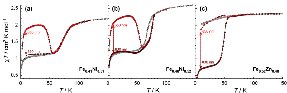
Figure 5. Temperature dependence of the \chi T product (measured in the dark and at 0.4 \text{ K min}^{-1} ) for \text{Fe}_{0.41}\text{Ni}_{0.59} (a; 0.1 T), \text{Fe}_{0.48}\text{Ni}_{0.52} (b; 0.1 T), and \text{Fe}_{0.52}\text{Zn}_{0.48} (c; 1 T) is shown in gray upon cooling down to 10 K. After cooling down the samples at 10 K in the dark, the red \chi T vs T data points were obtained after photoexcitation at 650 nm (at 10 \text{ mW cm}^{-2} , 1 h) for \text{Fe}_{0.41}\text{Ni}_{0.59} (a) and \text{Fe}_{0.48}\text{Ni}_{0.52} (b), while for \text{Fe}_{0.52}\text{Zn}_{0.48} (c), successive photoexcitations at 830 nm (at 17 \text{ mW cm}^{-2} , 7 h) and 650 nm (at 15 \text{ mW cm}^{-2} , 30 min) were performed before the magnetic measurements. After cooling down the samples at 10 K in the dark, the brown \chi T vs T data points were obtained after photoexcitation at 830 nm (at 17 \text{ mW cm}^{-2} , 5 h) for \text{Fe}_{0.52}\text{Zn}_{0.48} (c) while successive photoexcitations at 650 nm (at 10 \text{ W cm}^{-2} , 1 h) and at 830 nm for \text{Fe}_{0.41}\text{Ni}_{0.59} (a; at 10 \text{ mW cm}^{-2} during 2 h) and for \text{Fe}_{0.48}\text{Ni}_{0.52} (b; at 17 \text{ mW cm}^{-2} during 5 h) were performed before the magnetic measurements.
