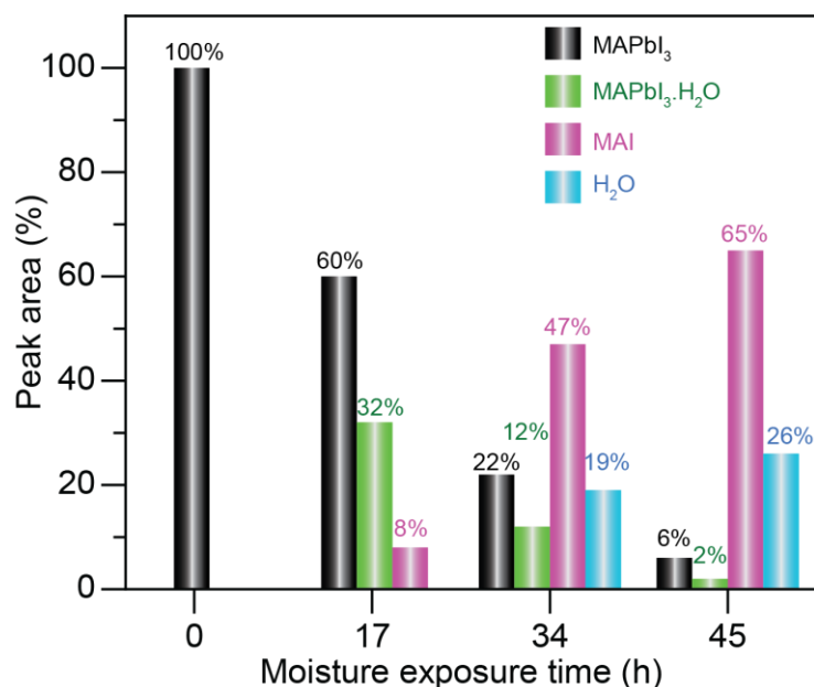
Figure 2. A plot of proton peak intensities of MAPbI 3 as a function of moisture exposure time for the different by products formed, which are color coded as depicted in the inset.
