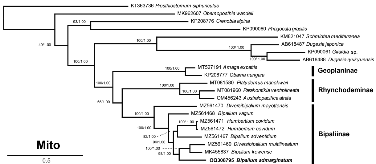
FIGURE 6. Maximum likelihood phylogenetic tree obtained from concatenated amino-acid sequences of the mitochondrial proteins of Bipalium admarginatum and other flatworms. The tree represents both Maximum likelihood and Bayesian inference phylogenies, performed using mtZOA+I+G4 and CPREV+I+G4 models of evolution, respectively. The tree with the best likelihood is shown, and bootstrap values are indicated. The BI tree had an identical topology, posterior probabilities are indicated on the right as decimal values. Subfamilies of Geoplanidae are indicated on the right. Based on the matrix and method used in Gastineau et al. (2022) with addition of the new sequence of B. admarginatum .
