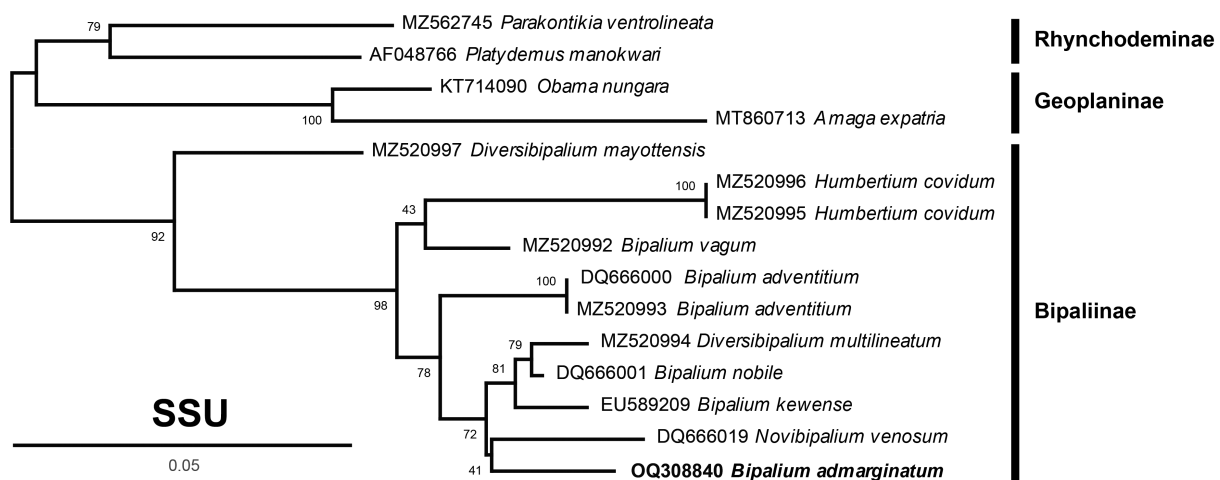
FIGURE 7. 18S phylogenetic tree of bipaliine geoplanids. Maximum likelihood phylogenetic tree based on 15 partial 18S genes, using the TVM+I+G4 model of evolution. The tree with the best likelihood is shown, and ML bootstrap support values are indicated. The subfamilies within the Geoplanidae (Rhynchodeminae, Geoplaninae and Bipaliinae) are indicated. Based on the matrix and method in Justine et al. (2022) with the addition of the new sequence of Bipalium admarginatum .
