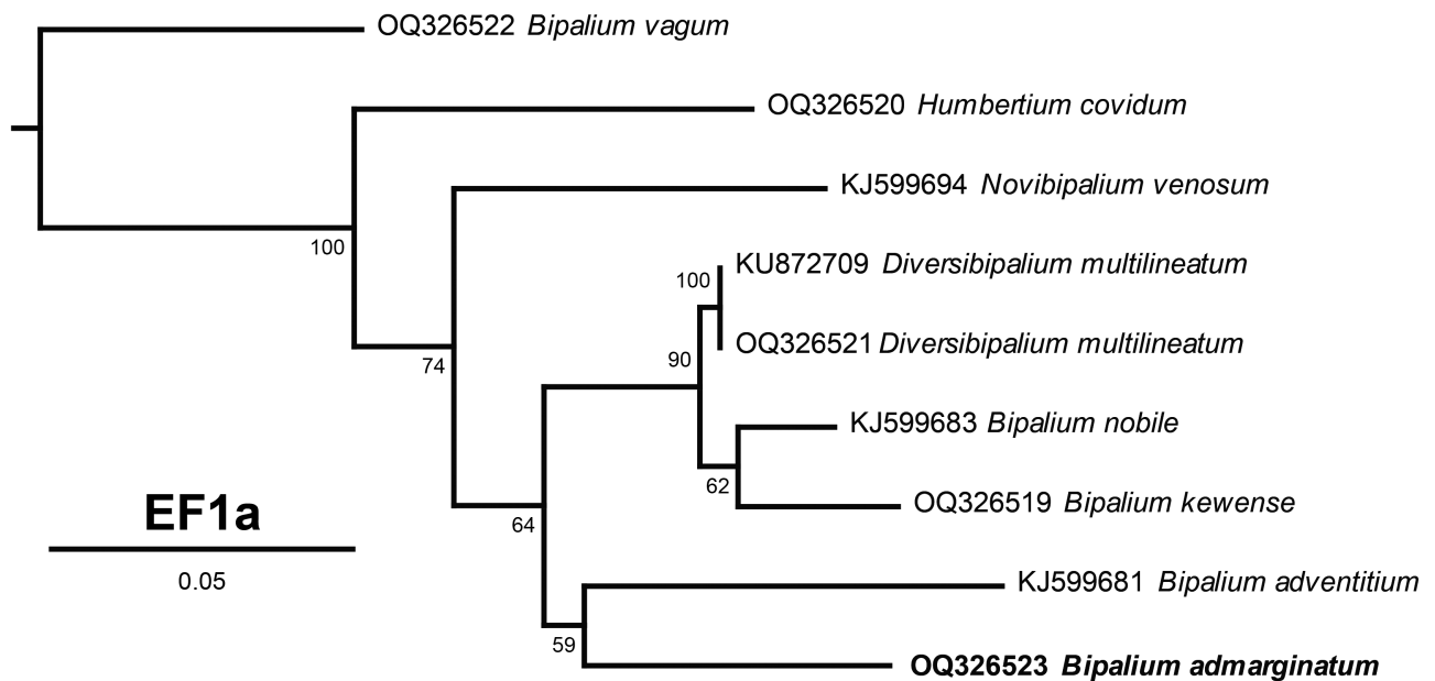
FIGURE 8. Phylogenetic tree of geoplanids based on nine sequences of elongation factor 1-alpha ( EF1-a ), including five new; only the part of the tree containing the Bipaliinae is shown. Maximum likelihood phylogenetic tree based on 9 sequences, using the GTR+I+G4 model of evolution. All OQ sequences are our own and new.
