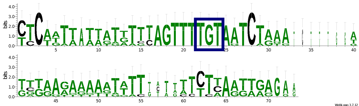
FIGURE 5. Sequence motifs obtained by aligning with WebLogo3 the tRNA-Thr genes annotated in the mitogenomes of Diversibipalium multilineatum , Bipalium kewense , Diversibipalium mayottensis , Bipalium vagum , Obama nungara and Amaga expatria with the suspected corresponding sequences of Humbertium covidum and Bipalium admarginatum . The height of each nucleotide indicates the conservation at that position. The blue box shows the conserved sequence of the anticodon.
