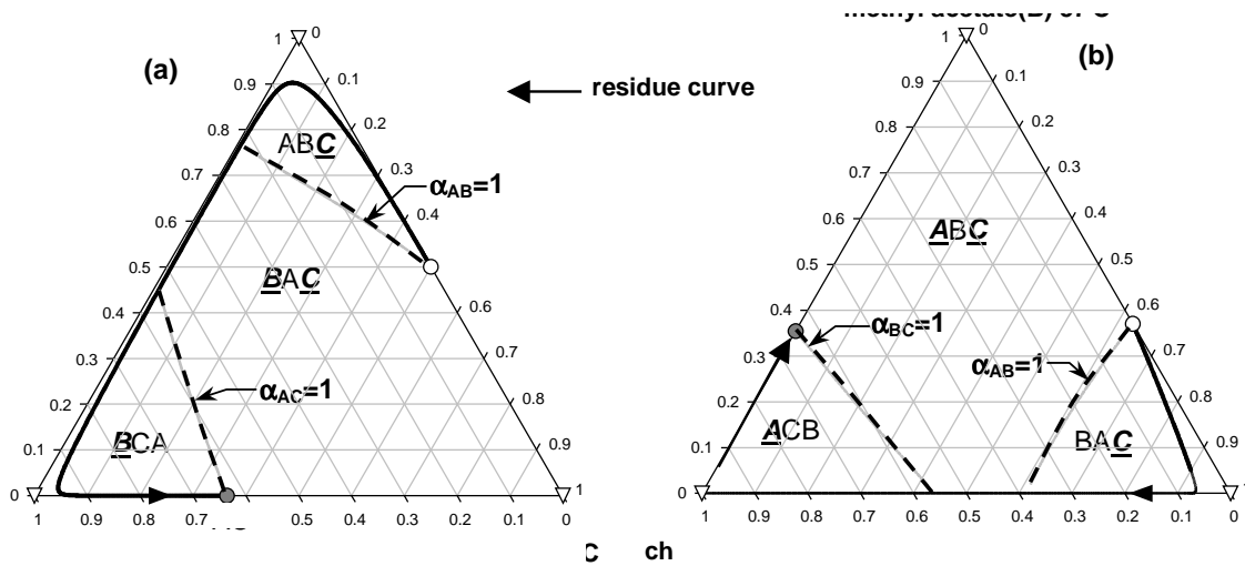
Figure 2. Residue curve map and univolatility lines for mixtures of diagram 2.0-1
