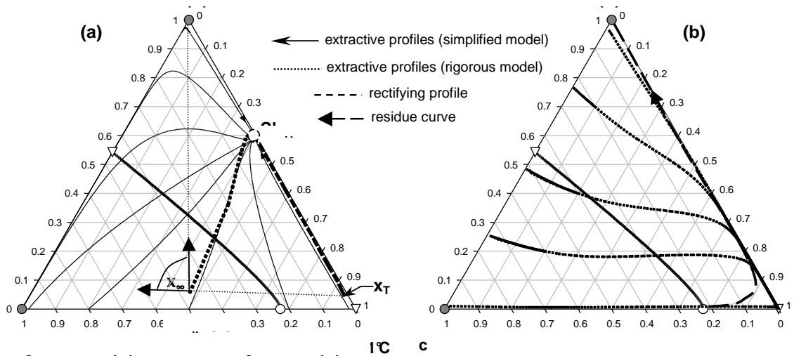
Figure 5. Map of extractive liquid profiles. (a). Batch rectifier for B. (b) Batch stripper for C.
