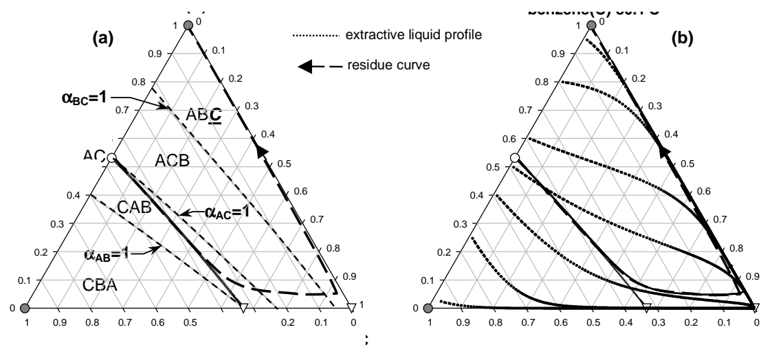
Figure 6. (a)Residue curve map and univolatility lines for mixtures of diagrams 2.0-2b. (b) Map of extractive liquid profiles for component B in a batch stripper.
