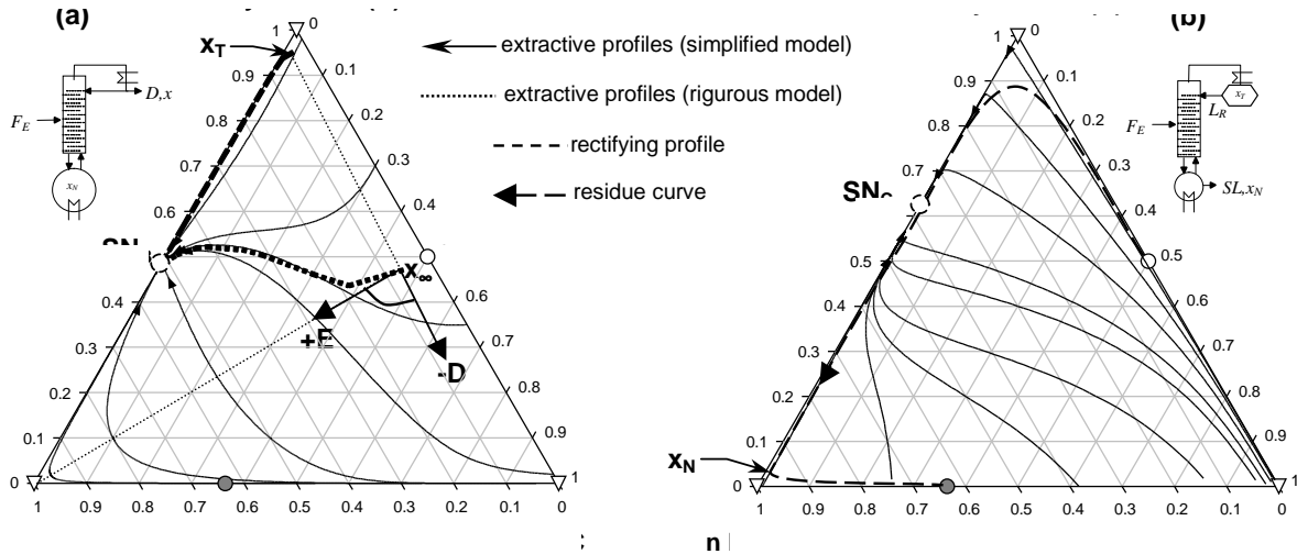
Figure 3. Map of extractive liquid profiles. (a) Batch rectifier for B . (b) Batch stripper for C
