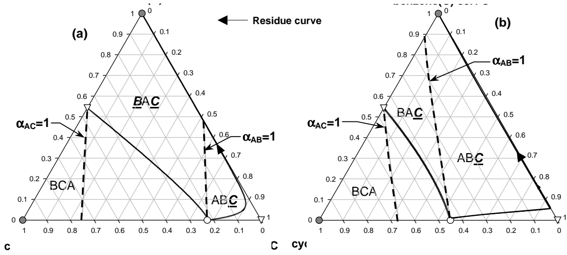
Figure 4. Residue curve map and univolatility lines for diagram 2.0-2b mixtures
