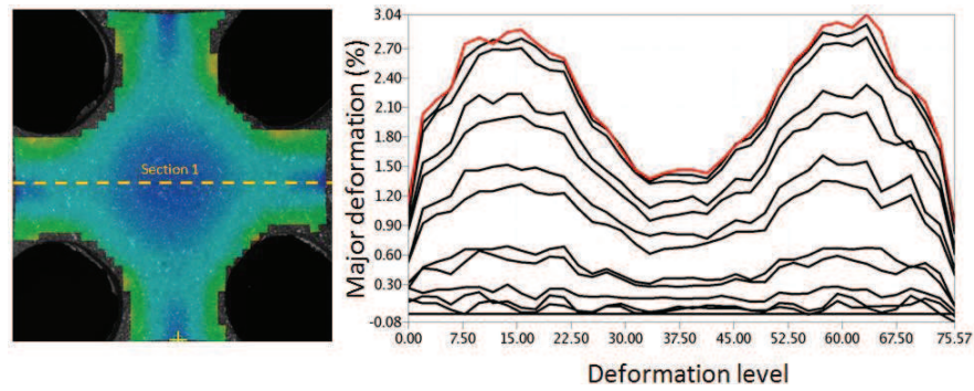
Fig. 12. Distribution of major deformation (%) along Section 1
