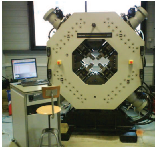
Fig. 1. Instron 8800 bi-axial fatigue tensile machine
