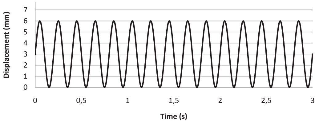
Fig. 6. Sinusoidal displacement cycle
