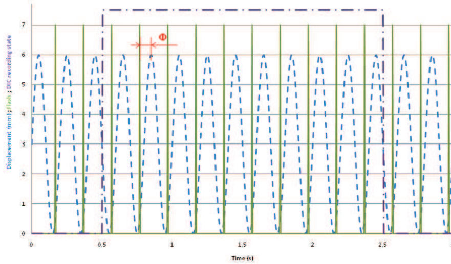
Fig. 7. Graph of synchronization issue
