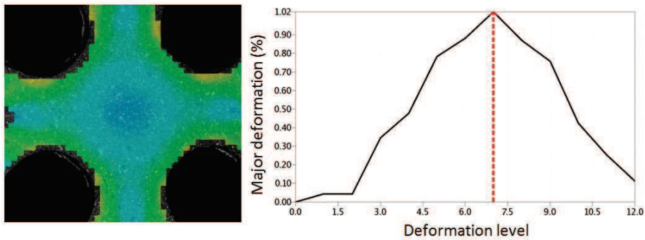
Fig. 10. Major deformation (%) at the maximum amplitude
