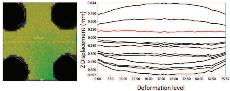
Fig. 13. Distribution of out of plane Z displacement (mm) along Section 1
