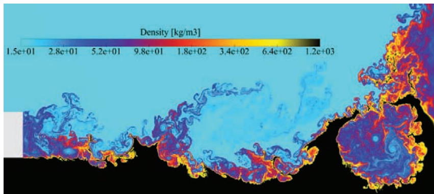
Figure 4. Density field, ranging from 15 \text{ kg}\cdot\text{m}^{-3} (blue) to 1200 \text{ kg}\cdot\text{m}^{-3} (black) using a logarithmic scale.
