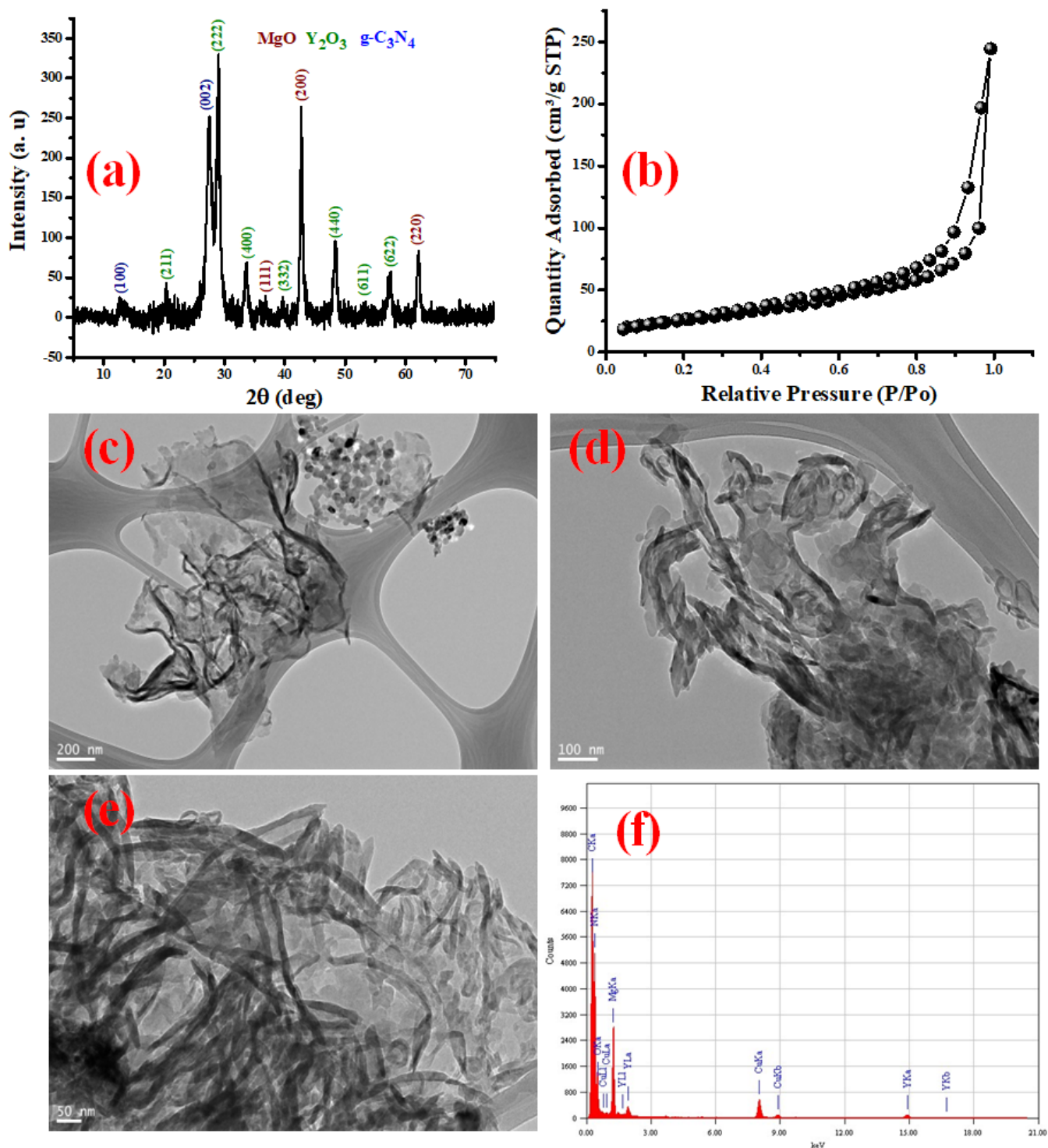
Figure 1. (a) XRD pattern; (b) BET surface area graph; (c–e) TEM images with different magnifications; and (f) EDX of MgY 2 O 4 @g-C 3 N 4 nanomaterials.
