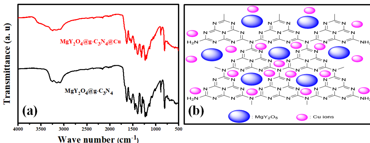
Figure 9. (a) FTIR spectra of MgY 2 O 4 @g-C 3 N 4 nanomaterials previously and after Cu (II) adsorption; and (b) proposed adsorption mechanism.
