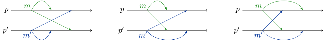
(a) Pattern MP1: forbidden by MBroadcast and by PBroadcast
