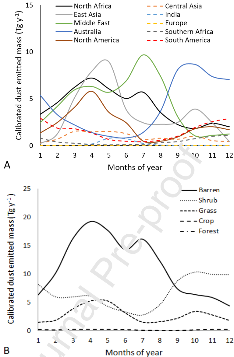
Figure 7. Total (2001-2020) monthly calibrated albedo-based dust emission seasonality ( F_{\text{cal}} ; Tg y -1 ) stratified by global region (A) and by land cover (B). See Figure 4 for definition of global regions and global land covers used in this study.
