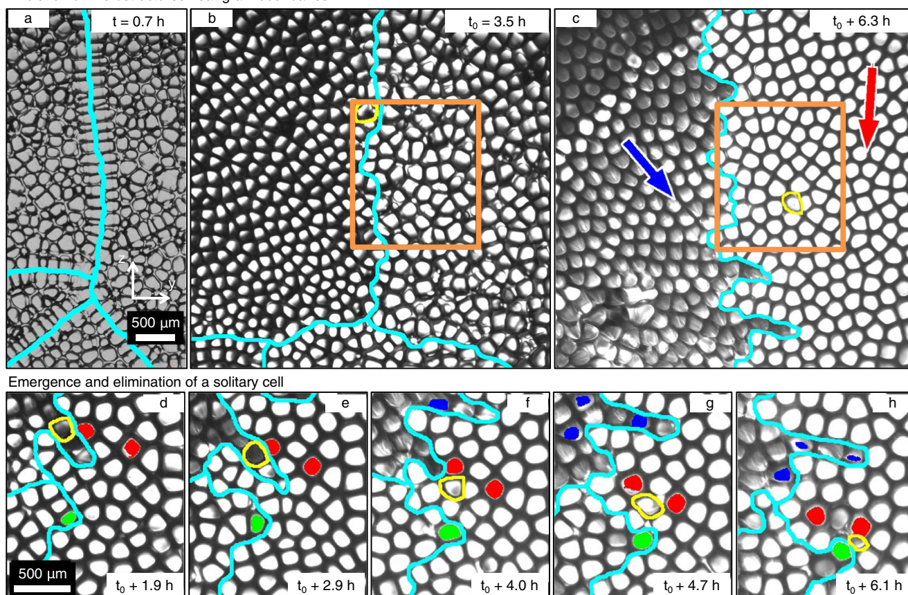
Fig. 1 | Evolution of the solid-liquid interface pattern, grain boundaries, and emergence of solitary cells. The interface is seen from its liquid side during directional solidification experiments in microgravity at different times t . Grain boundaries (GBs) appear in cyan lines. The GBs have a uniform linear morphology at early time in (a). A solitary cell (SC), outlined in yellow, emerges in the orange
