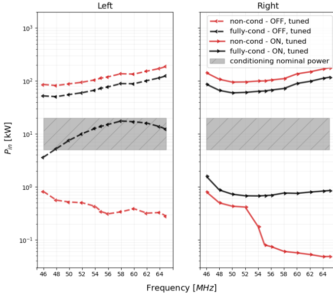
Fig. 11. The right -side generator’s forward powers, as a function of the ICRH frequency range, responsible for triggering the multipactor in the different antenna sides (the figure of left (right) corresponds to the results of the left (right) side of the antenna). The red (respectively black) curves correspond to the minimal and maximal forward powers of the on-mode generator, triggering multipactor in one antenna side for the non-conditioned (fully conditioned) TEEY data curve represented in red (black) in Fig. 2. The dashed grey band corresponds to the nominal RF conditioning operational powers.
