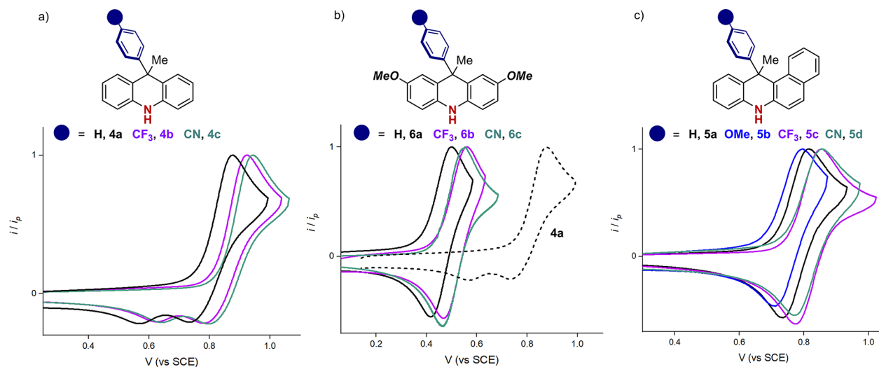
Figure 4. Normalized cyclic voltammograms of PCs 4a–c , 6a–c , and 5a–d . Potentials are reported in V vs SCE. Normalized cyclic voltammograms of PCs 6a–c (solid traces) compared with the normalized cyclic voltammogram of PC 4a (dashed trace).
