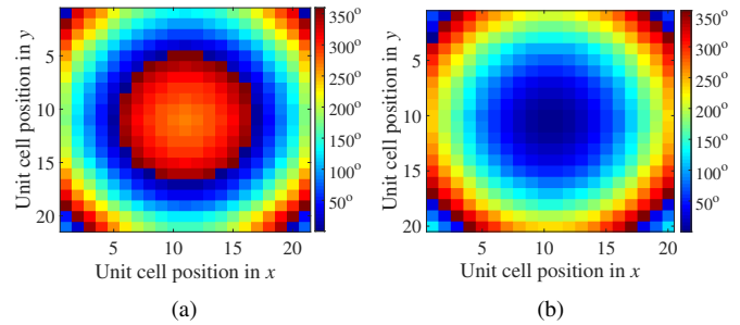
Fig. 10. Phase maps in reflectarray at 41 GHz: (a) for V-pol and, (b) for H-pol.
