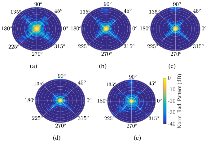
Fig. 17. Measured 3-D LHCP at different frequencies: (a) 32 GHz, (b) 36.5 GHz, (c) 41 GHz, (d) 45.5 GHz and, (e) 50 GHz. The radial lines mark the azimuth angles \phi while the concentric circles mark the elevation angles \theta . The angular distance between each concentric circle is 10^\circ .
