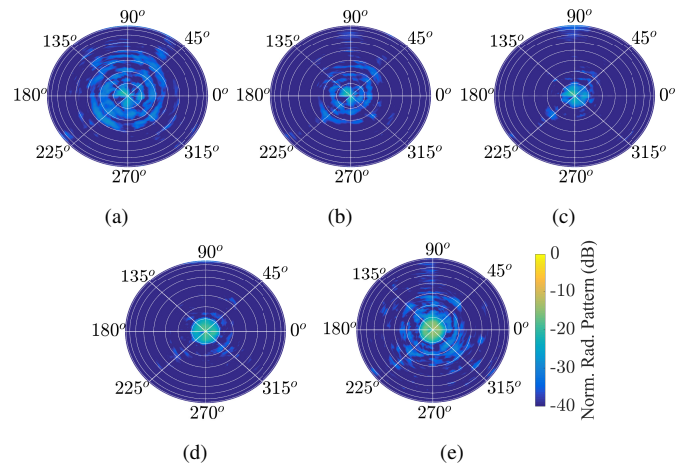
Fig. 18. Measured 3-D RHCP at different frequencies: (a) 32 GHz, (b) 36.5 GHz, (c) 41 GHz, (d) 45.5 GHz and, (e) 50 GHz. The angle of the radial lines mark the azimuth angles \phi while their intersection with the concentric circles mark the elevation angles \theta . The angular distance between each concentric circle is 10^\circ .
