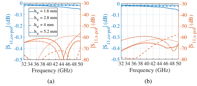
Fig. 3. Co-polarized and cross-polarized reflection in magnitude of the RA unit cell (3) in: (a) normal incidence and, (b) oblique incidence ( \phi = 90^\circ and \theta = 20^\circ ).
