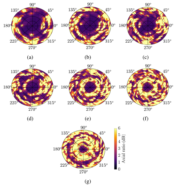
Fig. 19. Measured 3-D axial ratio at different frequencies: (a) 32 GHz, (b) 35 GHz, (c) 38 GHz, (d) 41 GHz, (e) 44 GHz, (f) 47 GHz and, (g) 50 GHz. The angle of the radial lines mark the azimuth angles \phi while their intersection with the concentric circles mark the elevation angles \theta . The angular distance between each concentric circle is 5^\circ .
