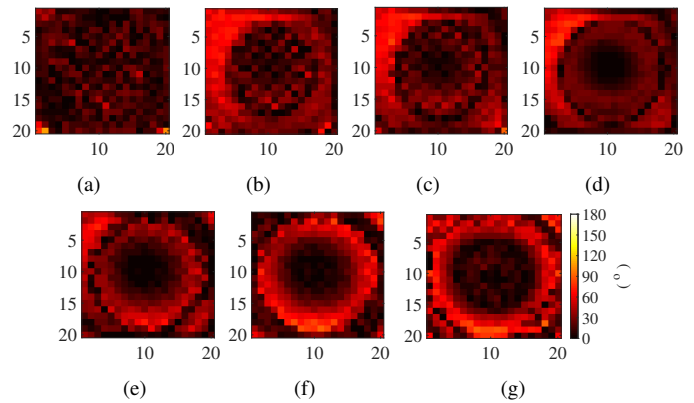
Fig. 14. Error phase maps for H-pol at different frequencies: (a) 32 GHz, (b) 35 GHz, (c) 38 GHz, (d) 41 GHz, (e) 44 GHz, (f) 47 GHz and, (g) 50 GHz.
