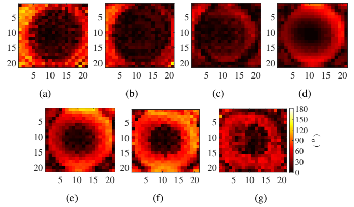
Fig. 13. Error phase maps for V-pol at different frequencies: (a) 32 GHz, (b) 35 GHz, (c) 38 GHz, (d) 41 GHz, (e) 44 GHz, (f) 47 GHz and, (g) 50 GHz.
