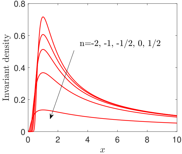
FIG. 5. Invariant density defined in Eq.(61) for the geometric Brownian motion with nonlinear drift. We used the parameters H_0=1 , G_0=1 and a variable exponent n .
