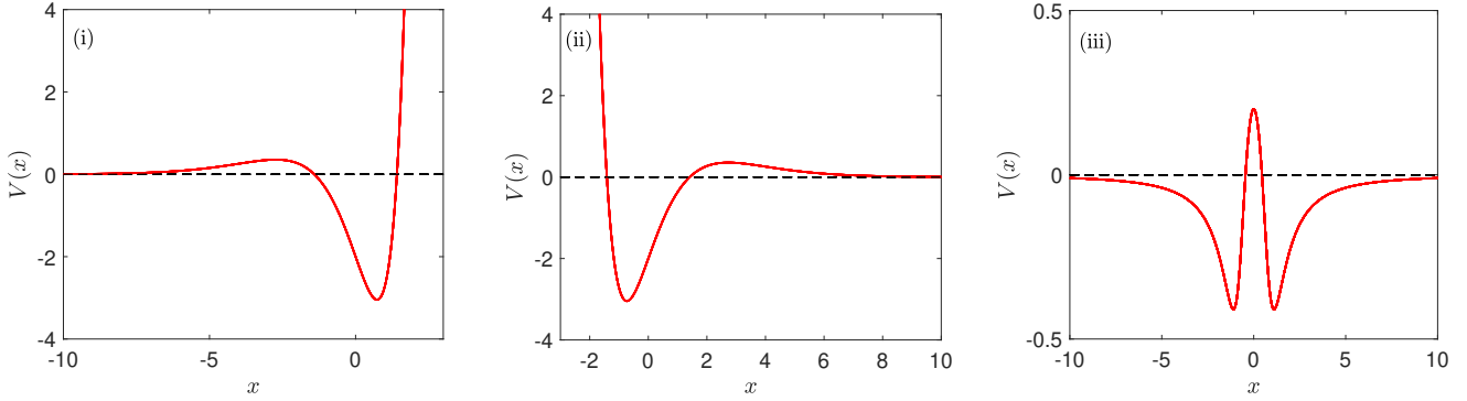
FIG. 4. Three examples of potential energy involving infinite ergodicity: (i) non-confining on the left, \lim_{x \rightarrow -\infty} V(x) = 0 and \lim_{x \rightarrow +\infty} V(x) = +\infty ; (ii) non-confining on the right, \lim_{x \rightarrow -\infty} V(x) = +\infty and \lim_{x \rightarrow +\infty} V(x) = 0 ; (iii) non-confining on both the left and the right, \lim_{x \rightarrow -\infty} V(x) = 0 and \lim_{x \rightarrow +\infty} V(x) = 0 .
