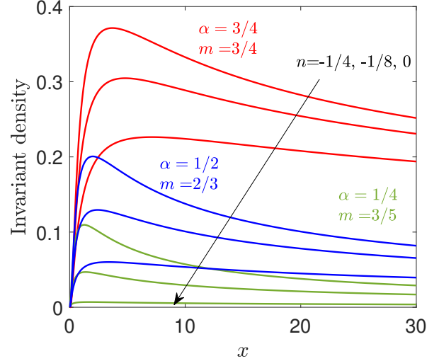
FIG. 8. Invariant density defined in Eqs.(89) and (90) for the generalized geometric Brownian motion with nonlinear drift. We used the parameters H_0 = -1 , G_0 = 1 , variable exponents n and m , and variable parameter \alpha .
