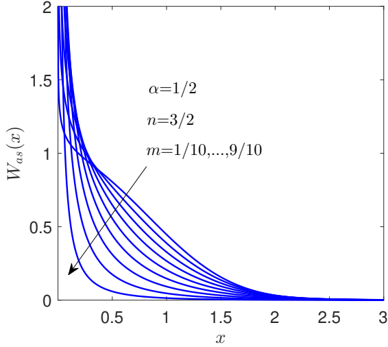
FIG. 6. Example of asymptotic distributions in the region defined by Eq.(73). We implemented Eq.(76) with the parameters H_0 = 3/2 and G_0 = 1 .
