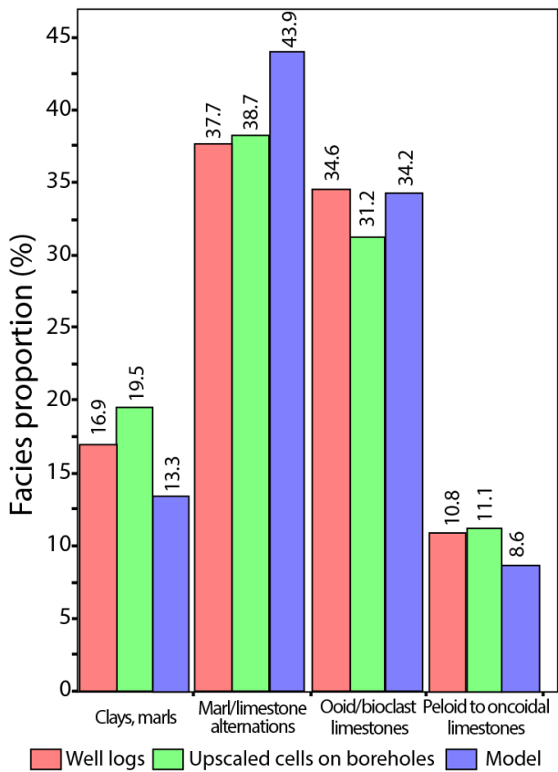
645 Figure 11. Facies association proportion in well logs, in upscaled cells along each well and in the entire model (12.2 million 646 cells).
