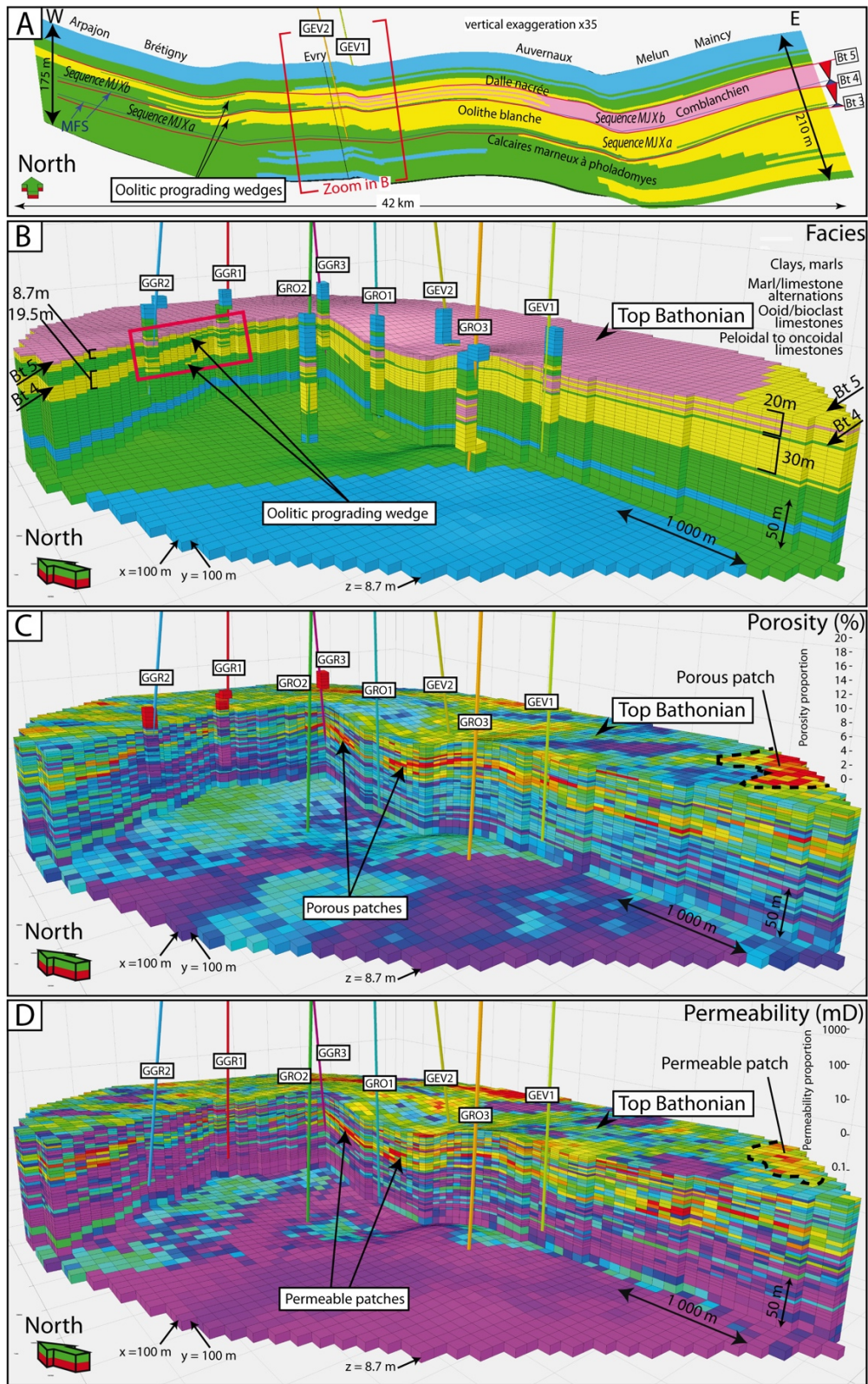
1097 Figure 21. Close look at the zone of the Grigny Bathonian reservoir highlighted in Fig 3. A- West-east stratigraphic cross-section through the modeled area, crossing near cities of Arpajon, Brétigny, Evry, Auvernaux and Maincy. The two main 1098 reservoir sequences MJXa and MJXb prograde westward. B- Facies distribution. C- Porosity distribution. D- Permeability 1099 distribution. The red rectangle highlights the reservoir thinning discussed in the main text.
