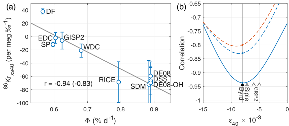
Figure 3. Calibrating Kr-86 excess. (a) ^{86}\text{Kr}_{\text{xs}} as a function of \Phi for the calibration dataset. Circles give the site mean, and the error bars denote the \pm 1\sigma standard deviation between samples (uncertainty in corrections and measurements not included). The number of samples at each site is given in Table 1. The Pearson correlation coefficient is r = -0.94 when considering site data means and r = -0.83 when considering all individual samples. Data are corrected for gas loss using \epsilon_{40} = -0.008 (Appendix A1) and corrected for thermal fractionation using site mean ^{15}\text{N} excess (Appendix A2). The calibration curve for ^{86}\text{Kr}_{\text{xs}15} is identical in this case, with slightly larger error bars. (b) Correlation of the calibration curve as a function of the gas loss correction scaling parameter \epsilon_{40} . The solid line gives the correlation for both site mean ^{86}\text{Kr}_{\text{xs}15} and ^{86}\text{Kr}_{\text{xs}40} (identical); the dashed lines show the correlation using individual samples for ^{86}\text{Kr}_{\text{xs}40} (blue) and ^{86}\text{Kr}_{\text{xs}15} (orange). Triangles denote the \epsilon_{40} estimate from the Byrd, Siple, and GISP2 ice cores (Fig. A2; Kobashi et al., 2008a; Severinghaus et al., 2003).
