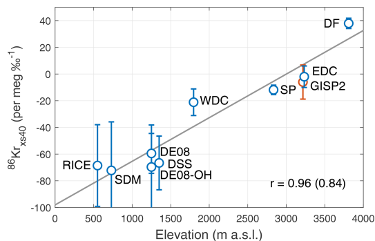
Figure A6. Kr-86 excess dependence on site elevation. The vertical axis is the ^{86}\text{Kr}_{\text{xs}} . The linear fit has a slope of 34 \text{ per meg } \%^{-1} per 1000 m elevation.
