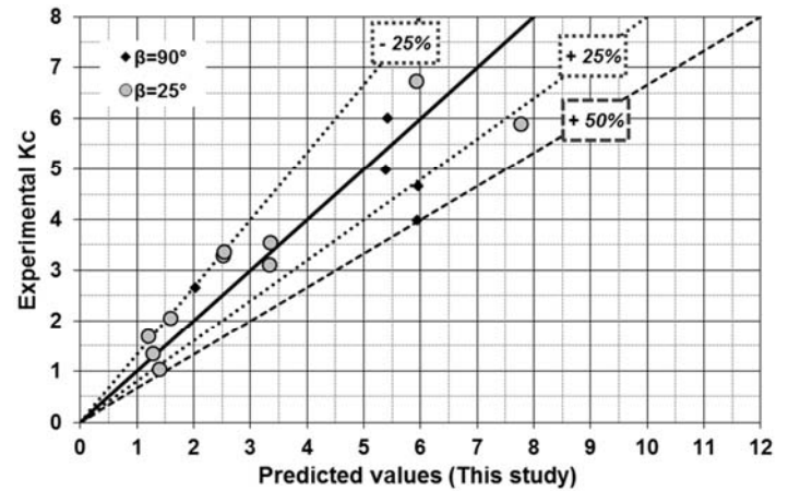
Figure 8 : Comparison between experimental K_C values and those predicted by Eq. 10 in this study.
