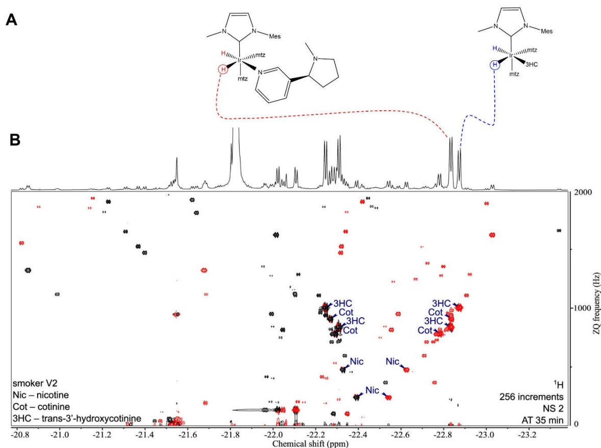
(A) Illustration of hyperpolarized hydrides showing different chemical shifts in function of bond metabolites, Cotinine (left, red) and 3HC (right, blue) (B) 2D ZQ p -H 2 spectrum of urine extract in CDCl 3 . Each complex of an analyte gives rise to two opposite phase doublets at the same ZQ frequency. Chiral analytes (i.e., Nic, Cot, and 3HC) can combine in two ways due to stereogenic center on iridium in the complex, forming two diastereomers with different physical properties. Signals were assigned by internal standard addition during method development. Upper 1D trace recorded separately with the 1D Selective excitation of polarization using PASADENA (SEPP) sequence. Adapted from reference [63●●].
