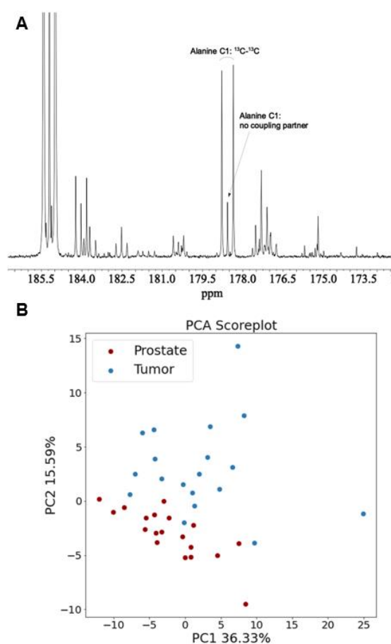
(A) Carbonyl region of hyperpolarized 1D- ^{13}\text{C} NMR spectrum of prostate extract from mouse injected with [\text{U-}^{13}\text{C}] glucose 30 min prior to tissue harvest. (B) Full Spectrum analysis of hyperpolarized 1D ^{13}\text{C} NMR spectra by principal component analysis (PCA) each point represents a single sample of which are determined by the collective contributions of all sample corresponding integrals. Data was mean centered and unit variance scaled before PCA was applied. Adapted from reference [35●●].
