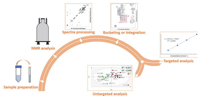
Figure 5. Typical workflow for untargeted or targeted metabolomics using 2D NMR. Reproduced from Ref. 81 .
