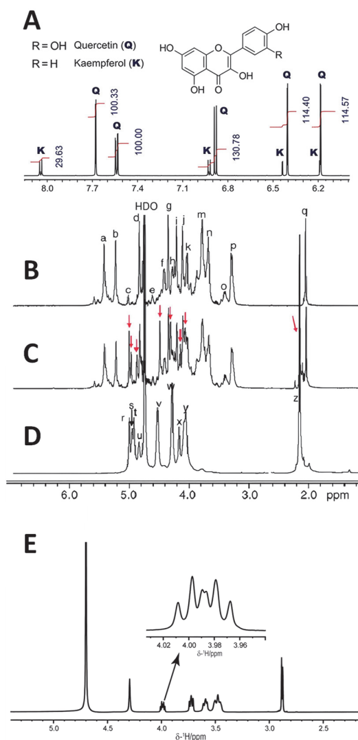
Figure 1. 1 H NMR spectroscopy examples illustrating the complexity of mixtures and of their quantification in pharmaceutical industry. (A) Application of the relative (100%) qHNMR. A commercial sample of quercetin (Q; declared purity >99%; 24.67 mg/mL [not required for purity calculation] in DMSO- d 6 , 600 MHz) was analyzed. A structurally related compound, kaempferol (K), was identified as an impurity. On the basis of the relative integral ratios, the content of quercetin and kaempferol in the sample was determined as 87.8% and 12.2% w/w, respectively. (B, C, D) 1 H-NMR spectra acquired at 800 MHz and assignment of heparin, contaminated heparin and OSCS contaminant. (B) 1 H-NMR spectrum of heparin. a, H1 GlcNS, GlcNS6S; b, H1 IdoA2S; c, H1 IdoA; d, H5 IdoA2S; e, H1 GlcA; f, H6 GlcNS6S; g, H2 IdoA2S; h, H6' GlcNS6S; i, H3 IdoA2S; j, H4 IdoA2S; k, H5 GlcNS5S; l, H6 GlcNS; m, H4 GlcNS6S; n, H3 GlcNS, GlcNS6S; o, H2 GlcA; p, H2 GlcNS6S; q, acetyl CH 3 . (C) 1 H-NMR spectrum of contaminated heparin; peaks with red arrows show peaks not observed in heparin. (D) 1 H-NMR spectrum of OSCS contaminant. r, H4 GalNAc2S4S6S; s, H3 GlcA2S3S; t, H1 GlcA2S3S; u, H1 GalNAc2S4S6S; v, H2 and 4 of GlcA2S3S; w, H6 GalNAc2S4S6S; x, H5 GlcA2S3S; y, H2,3 and 5 GalNAc2S4S6S; and z, acetyl CH 3 of GalNAc2S4S6S. (E) Conventional 1D- 1 H NMR spectrum of aspartic acid (1 eq) containing CSA (–)-(18-Crown-6)-2,3,11,12-tetracarboxylic acid (0.25eq) in solvent D 2 O. (A) Reproduced with permission from Ref. 30 . (B, C, D) Reproduced with permission from Ref. 31 . (E) Reproduced with permission from Ref. 32
