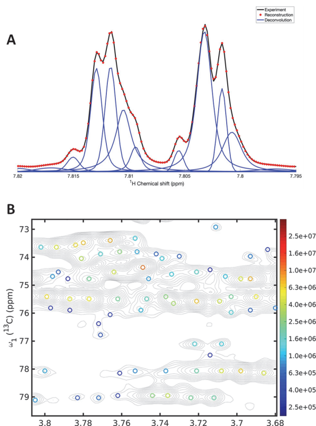
Figure 3. Potential of machine-learning methods for the decomposition of complex overlapped spectra in 1D NMR metabolomics. (A) Application of DEEP Picker1D and Voigt Fitter1D to a spectral region of the 1D ^1\text{H} spectrum of mouse urine. Experimental and reconstructed spectra are depicted as black lines and red dots, respectively. Deconvoluted individual peaks are depicted as blue lines. The deconvolution by DEEP Picker1D was performed with model 2 with a PPP number of 8. (B) Illustration of performance of DEEP Picker for 2D ^{13}\text{C} - ^1\text{H} HSQC of mouse urine. DEEP Picker is able to identify and distinguish between cross-peaks that strongly overlap, which poses a significant challenge for their analysis by traditional peak pickers. Picked cross-peaks are indicated as circles and color-coded according to their amplitude on a logarithmic scale with logarithmic contour line spacings. (A) reproduced from Ref. 60 ; (B) reproduced from Ref. 22 .
