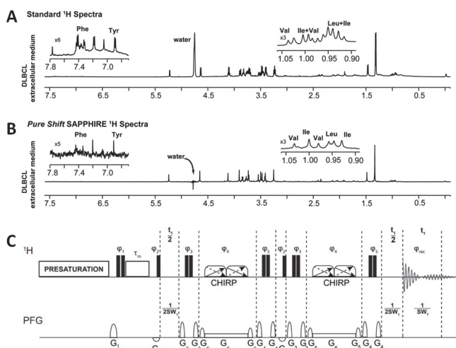
Figure 4. Potential of pure-shift 1 H NMR for metabolomics. Standard (A) and pure-shift SAPHIRE (B) 1 H NMR spectra recorded on DLBCL cancer extracellular medium. Regions of interest are magnified to show the evolution of proton lineshape. (C) Pulse sequence used to record pure-shift SAPHIRE 1 H NMR spectra. Reproduced with permission from Ref. 74 .
