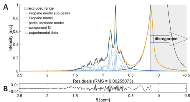
Figure 8. Analysis of a ^1\text{H} NMR gas spectrum. (a) Hard model for propane (7.7 mol%) mixed with methane (92.3 mol%) at 200 bar total pressure. (b) Fit residual showing that the model represents the measured signal with high accuracy. Reproduced with permission from Ref. 135
