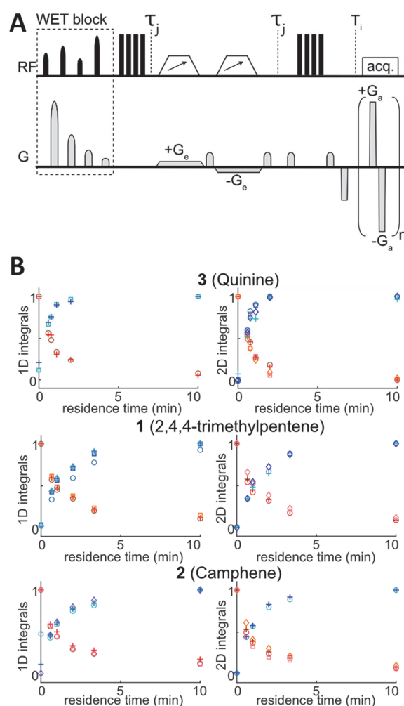
Figure 9. Illustration of the potential of UF 2D COSY for the in-line monitoring of flow photochemistry reactions, consisting of the thiol-ene addition of 2-mercaptoethanol to three unsaturated organic compounds: 2,4,4-trimethyl-1-pentene 1 , camphene 2 and quinine 3 (A) UF COSY pulse sequence used in this work, including a WET solvent suppression module combined with composite 90° pulses. (B) Integrals of selected reagent (red) and product (blue) correlations as a function of the residence time for the 6 reaction runs on compounds 1-3. Reproduced from Ref. 151
