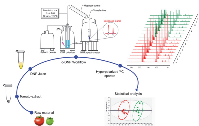
Figure 6. Illustration of untargeted metabolomics workflow on tomato extracts using 13 C d-DNP. Tomato extracts were prepared from a single pooled sample of tomato powder and mixed in a DNP juice (d8-gly: D2O: H 2 O, 6:3:1, v/v). 200 μL of solution were polarized at 1.2 K and 7.5 T using cross-polarization. Sample were dissolved with 5 mL of hot D 2 O, spectra were acquired after a total transfer time of 12.8 s. In spectra, letters a to h refer to red-ripe tomatoes, letters i to p refer to green tomatoes. Adapted from Ref. 100
