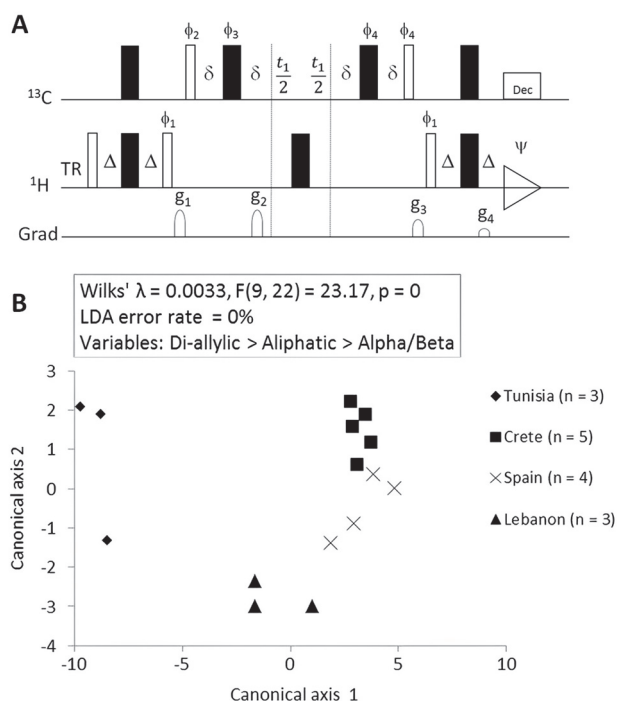
Figure 7. Application of high precision 2D HSQC NMR to isotopomics. (A)
