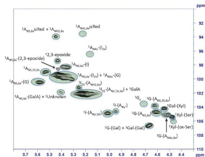
Figure 2. Heparin HSQC spectrum with signals assignments: region showing anomeric signals. Reproduced with permission from Ref. 43 .
