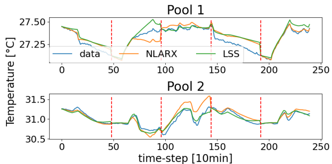
Fig. 8: Five 48 steps prediction on test data.
