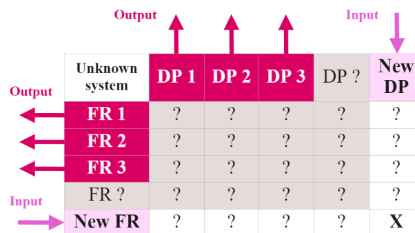
Figure 3. In Axiomatic Design, approaching an unknown system as a black box corresponds to having a series of matrix cells filled with question marks (gray cells), into which we input a new FR / DP pair (purple arrows). The new FR / DP pair has unknown couplings (white cells) since we do not know how they will interact with unclear existing FRs / DPs. Through a coupling propagation mechanism such as the one depicted in Figure 2, a series of FR / DP pairs that are impacted by the change, are called upon (red cells). This partial set of existing FR / DP pairs that were previously unclear, are the outputs of our black box system.
