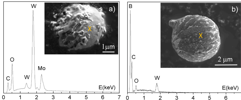
Fig. 4. a) W dominated spheroid containing C, O and Mo traces, size \sim 6 \mu\text{m} (C5 campaign). Molten W projections on the left side indicate that the dust temperature was close to that of a solid; b) B dominated spheroid containing C, O traces, size \sim 5 \mu\text{m} (C4 campaign). It was likely W before boronization.
