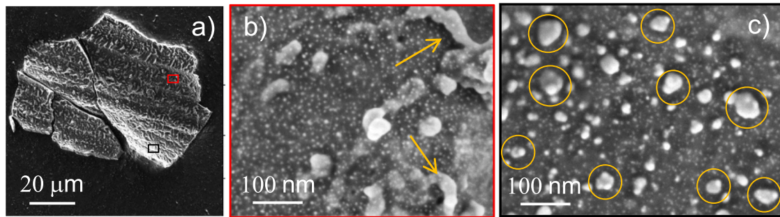
Fig. 8. a) piece of W coating of \sim 90 \mu\text{m} long and \sim 40 \mu\text{m} wide (C5 campaign); b) details of a whitish part made of dispersed NPs of \sim 5 \text{ nm} in the background (red square). Larger ones are either separated or melted with others to form chains (arrows); c) another whitish part (black square) still showing NPs of \sim 5 \text{ nm} in the background and bigger ones either separated or agglomerated (yellow circles). (For interpretation of the references to colour in this figure legend, the reader is referred to the web version of this article.)
