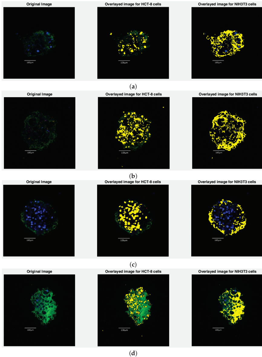
Figure 8. Overlay cluster and original images for HCT-8 and NIH3T3 cells: (a) 2:0.5 (2_05_z12), (b) 2:1 (2_1_z14), (c) 2:2 (2_2_z17), and (d) 2:4 (2_4_z10) ratio images.
