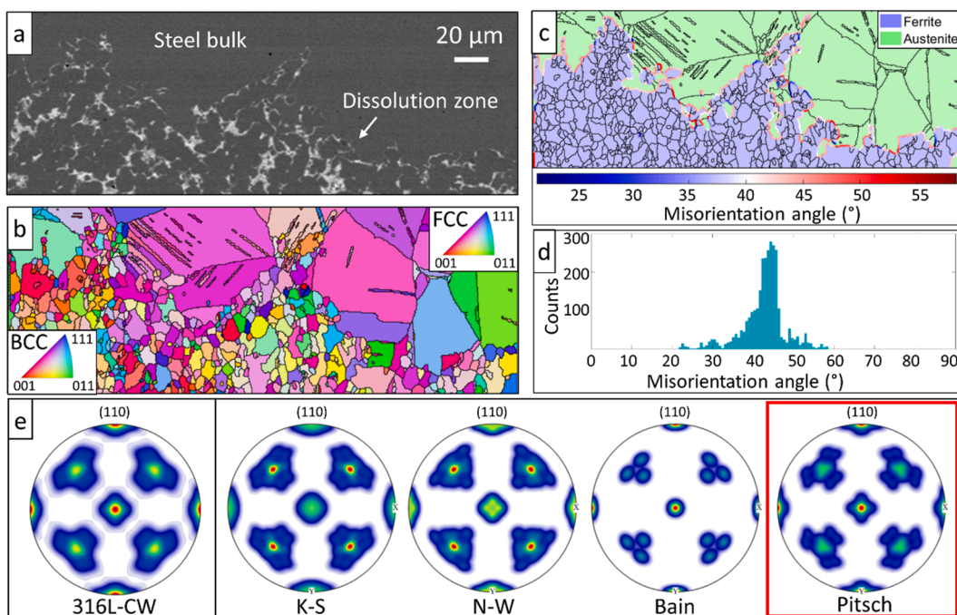
Fig. 3.48. (a) SEM † image of the ferritised dissolution-affected zone in a CW 316L AuSS exposed to oxygen-poor ( C_{\text{O}} \approx 10^{-9} wt%), static LBE at 550\text{ }^{\circ}\text{C} for 1000 h. (b) EBSD † orientation map with inverse pole figure colour maps for fcc and bcc phases. (c) EBSD phase map of the \gamma/\alpha interface misorientation boundary. (d) Misorientation angle distribution at the \gamma/\alpha interface boundary. (e) Estimated iso-density pole figures from experimental data and theoretical OR models in the (110) plane of the CW 316L AuSS. Adapted from [179].
