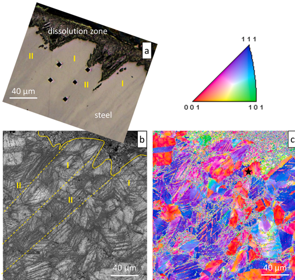
Fig. 3.47. (a) LOM † image of 60% CW 316L AuSS exposed to oxygen-poor ( C_{\text{O}} < 10^{-11} wt%), static LBE at 500\ ^\circ\text{C} for 1000 h: I – bands with higher Ni content, II – bands with lower Ni content. (b-c) EBSD † analysis shows that the segregation of defects is higher in the bands with lower Ni content. Adapted from [42].
