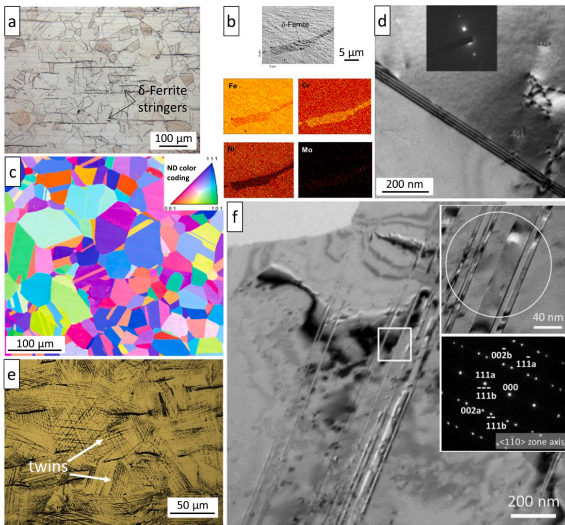
Fig. 2.4. Microstructure of SA † and CW † 316L AuSS. SA 316L: (a) LOM † image of \delta -ferrite stringers; (b) EDS † elemental maps of \delta -ferrite; (c) EBSD † grain orientation map; (d) TEM † BF image of nano-twins. CW 316L: (e) LOM image of deformation twins; (f) TEM BF images and SAED † pattern of deformation twins. Adapted from [40,58].
