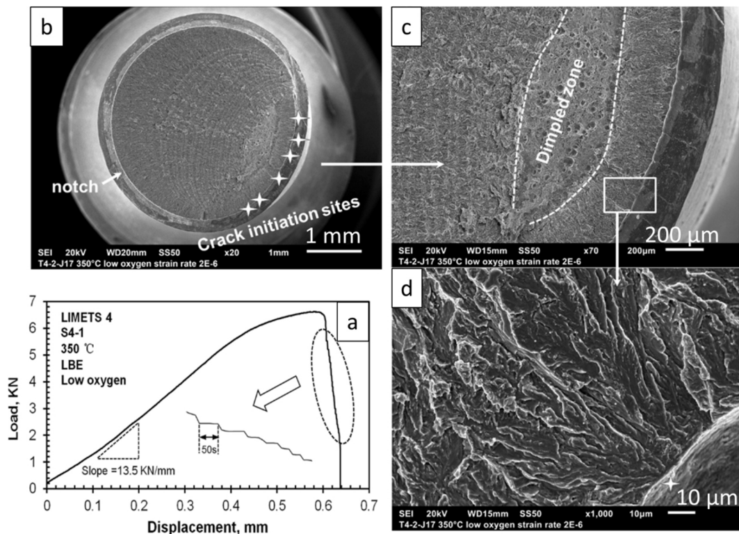
Fig. 4.41. SEM † images of T91 F/M steel fracture surfaces showing a mixture of LME-induced brittle fracture and ductile, dimple-rich fracture tested in low-oxygen liquid LBE at 350 ^{\circ} C. Adapted from [473].
