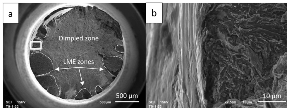
Fig. 4.33. SEM † images of the fracture surface of T91 F/M steels exposed to static liquid LBE: (a) dimpled zones are observed in the specimen centre and LME-affected zones in its periphery (outlined by white dashed curves), and (b) quasi-cleavage fracture appearance. Test conditions: 350 °C, oxygen-saturated LBE, \dot{\epsilon} \approx 5 \times 10^{-5} \text{ s}^{-1} . Adapted from [45].
