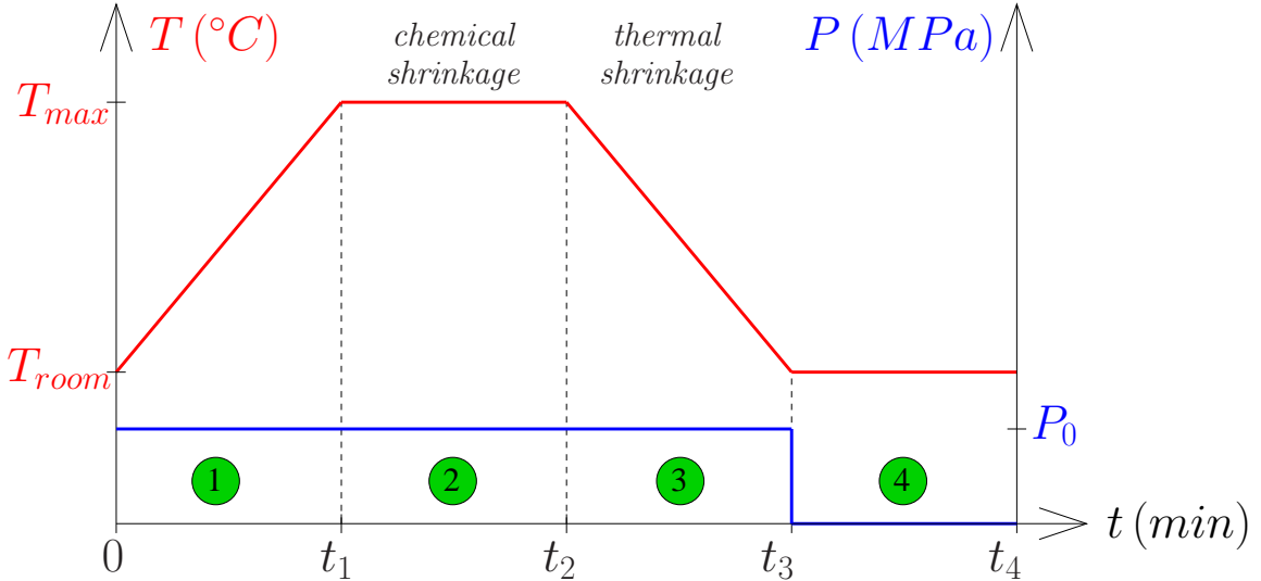
FIG. 1 – Schematic time evolution of the imposed temperature (left axis) and pressure (right axis) during manufacturing of PCB.
