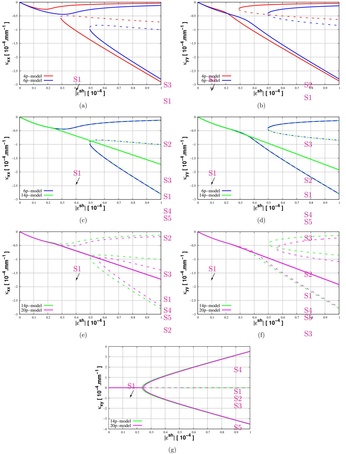
FIG. 4 – Evolution of curvatures as a function of the shrinkage strain |\varepsilon^{sh}| . Note that the average curvature predicted by the 20p-model is displayed in Figs. e-g). Material parameters are provided in Table 1. Dimensions of the bilayer plate are those of Fig. 3.
