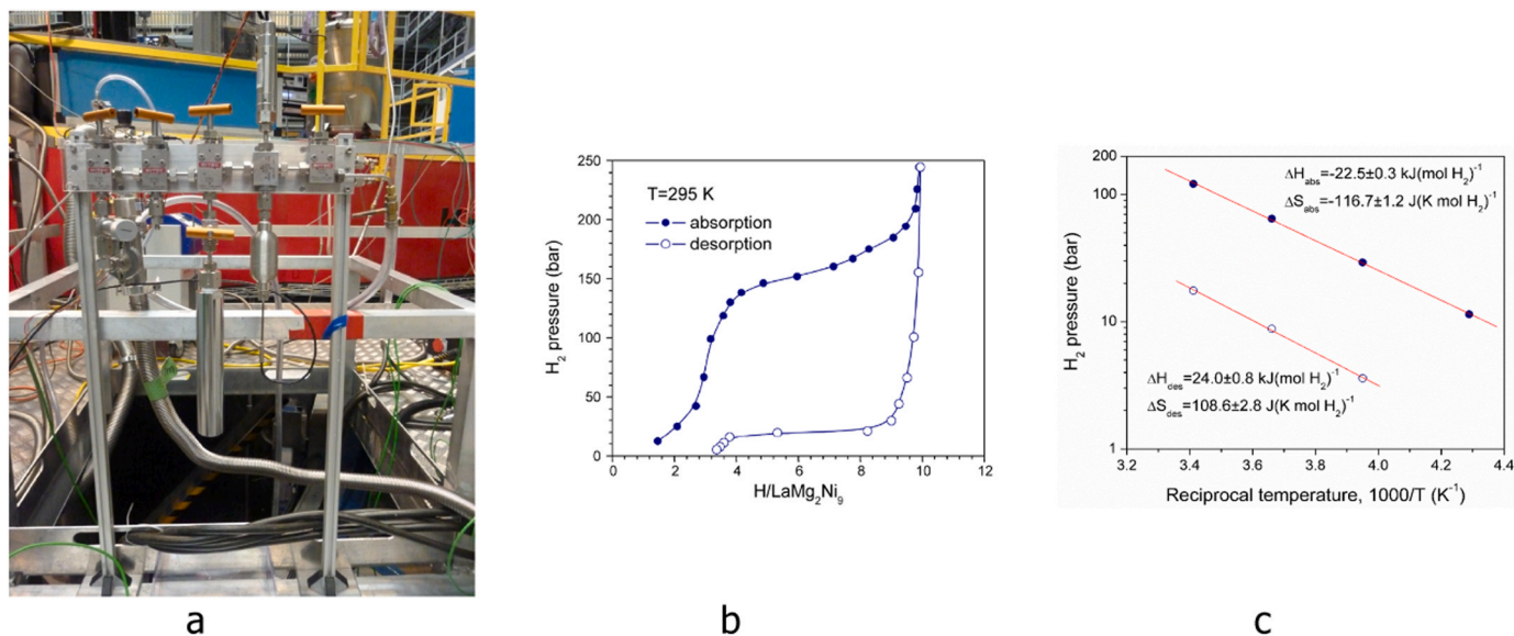
Fig. 27. (a) High pressure synthesis setup for the in situ NPD measurements at pressures up to 1000 bar D 2 ; (b) Room temperature isotherms of hydrogen absorption and desorption; van't Hoff plots (c) for La 1.09 Mg 1.91 Ni 9 -based hydride. At room temperature equilibrium pressure of hydrogen absorption is ~120 bar D 2 , while for the desorption P_{\text{eq}} equals to ~20 bar D 2 .
