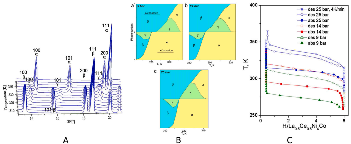
Fig. 20. (A) Temperature evolution of the in situ SR XRD pattern during hydrogen desorption from the \beta -La 0.5 Ce 0.5 Ni 4 CoH -6 hydride. Miller indices of the diffraction peaks for three constituent phases are shown. (B) Phase-structural composition of the La 0.5 Ce 0.5 Ni 4 Co-H 2 system from the refinements of the SR XRD data during isobaric desorption (upper part; heating) and absorption (lower part, cooling) with a heating/cooling rate of 2 K/min under isobaric conditions, 9 bar H 2 (a), 14 bar H 2 (b) or 25 bar H 2 (c). (C) Calculated isobars of hydrogen desorption and absorption built on the basis of the refined SR XRD data. (Reprinted with permission from [93]. Copyright (2010) Elsevier).
