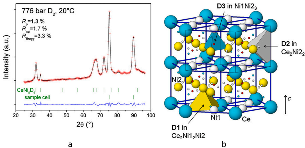
Fig. 25. (a) Refined neutron diffraction pattern for \text{CeNi}_5\text{D}_{6.3} (observed (+), calculated (—) and difference (bottom line) profiles). (b) Crystal structure of the \text{CeNi}_5\text{D}_{6.3} deuteride. Three types of interstices occupied by D atoms including tetrahedron \text{Ce}_2\text{Ni}_2 , trigonal bipyramid \text{Ce}_2\text{Ni}_3 and tetrahedron \text{Ni}_4 are shown. (Reprinted with permission from [39]. Copyright (2010) Elsevier).
