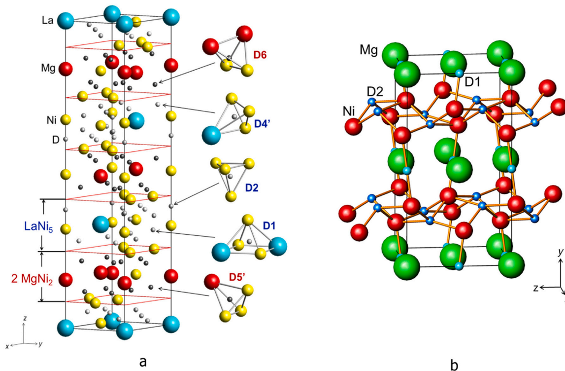
Fig. 28. (a) Crystal structure of \text{La}_{1 \pm 0.1}\text{Mg}_{2 \pm 0.1}\text{Ni}_9\text{D}_{9.4-9.5} and types of the filled interstices [110]; (b) The orthorhombic Cmca crystal structure of \text{MgNi}_2\text{D}_3 [111]. Two types of sites occupied by deuterium include a \text{Mg}_4\text{Ni}_2 octahedron for H1(D1) and a chair \text{Ni}_4 configuration for H2(D2) located within the buckled Ni-H nets containing bended spirals -\text{Ni}-\text{H}_2-\text{Ni}-\text{H}_2- . (Reprinted from an open access article [110] distributed under the Creative Commons Attribution license ( http://creativecommons.org/licenses/by/4.0/ )). (Reprinted with permission from [111]. Copyright (2015) Elsevier).
