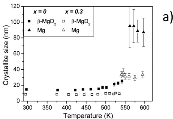
Fig. 33. (a) Evolution of the crystallite size of \beta - MgD_2 and Mg phases during thermal desorption (TD) of (1-x)MgD_2 - xTiD_2 samples with x=0 and 0.3. (b) Variation of TiD_2 cell volume during in situ TD and PCI measurements. Event ① corresponds to cell volume decrease during in situ TD. Events ② and ③ correspond to the cell volume variations during partial absorption and desorption of deuterium in TiD_2 phase at 548 K. (Reprinted with permission from [36]. Copyright (2013) American Chemical Society).
