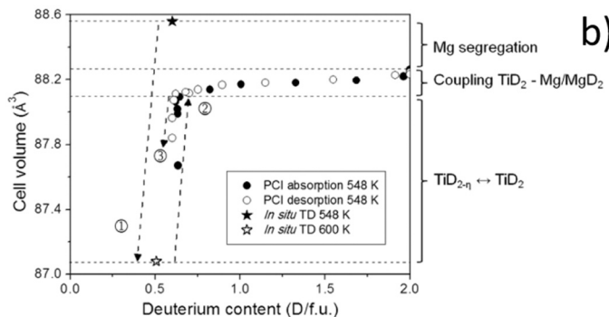
Fig. 33. (a) Evolution of the crystallite size of \beta - MgD_2 and Mg phases during thermal desorption (TD) of (1-x)MgD_2 - xTiD_2 samples with x=0 and 0.3. (b) Variation of TiD_2 cell volume during in situ TD and PCI measurements. Event ① corresponds to cell volume decrease during in situ TD. Events ② and ③ correspond to the cell volume variations during partial absorption and desorption of deuterium in TiD_2 phase at 548 K. (Reprinted with permission from [36]. Copyright (2013) American Chemical Society).
