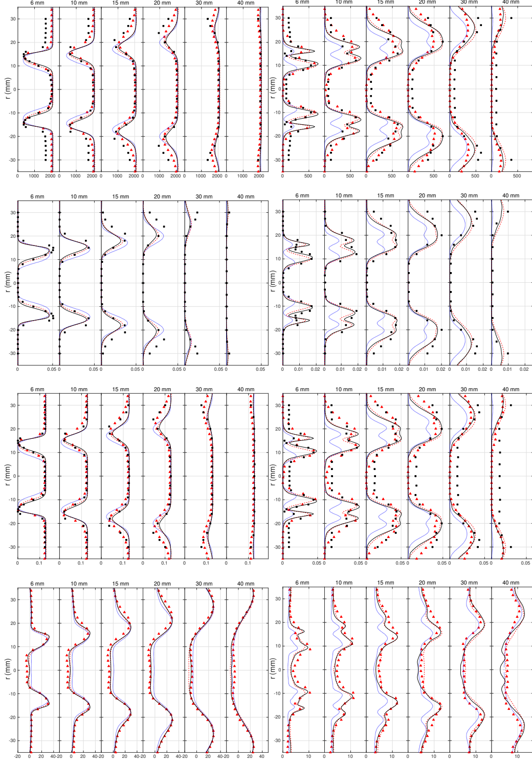
Figure 4: Quiet (or Stable) operating point 16 \phi = 0.83 . Average (left column) and RMS (right column) values at cut planes vertical to the burner axis in the combustion chamber. Temperature (K) , \text{CH}_4 , \text{CO}_2 , Axial velocity (m/s) (from top to bottom). Black solid squares (experimental), red solid triangles (YALES2 M_0 reference), blue dotted line ( M_0 ), red dashed line ( M_1 ) and black solid line ( M_2 )
