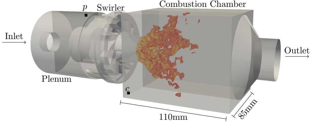
Figure 1: Global view of the PRECCINSTA setup along with the indication of the plenum ( p ) and chamber ( c ) probe locations.
