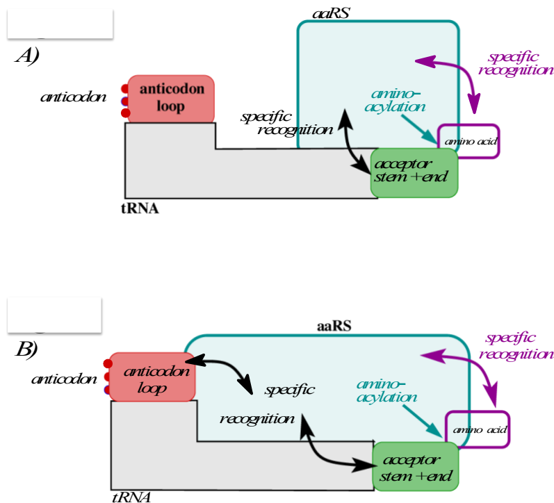
Figure 3 --- tRNA aminoacylation: the acceptor code
